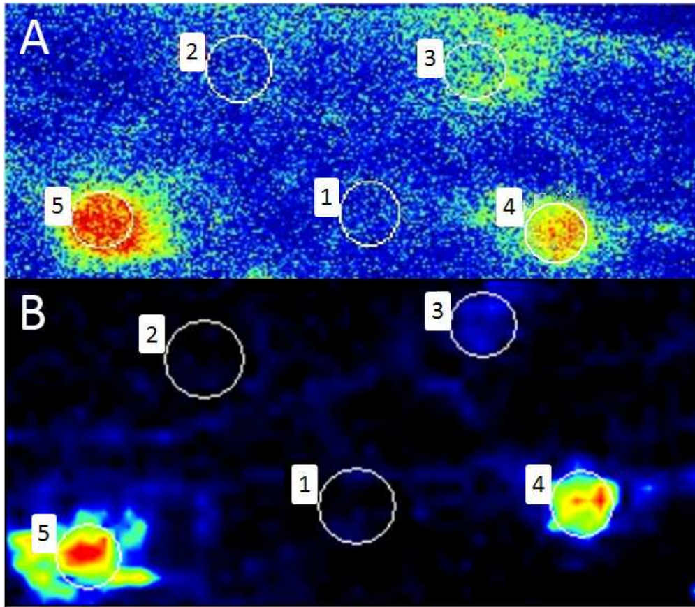
Measurement of skin blood flux on different skin sites of the forearm (numbered 1 to 5): unheated, heated to 36°C, to 39°C, to 42°C and to 44°C, respectively, using laser speckle contrast imaging (A) and laser Doppler imaging (B). 170x147mm (96 x 96 DPI)
