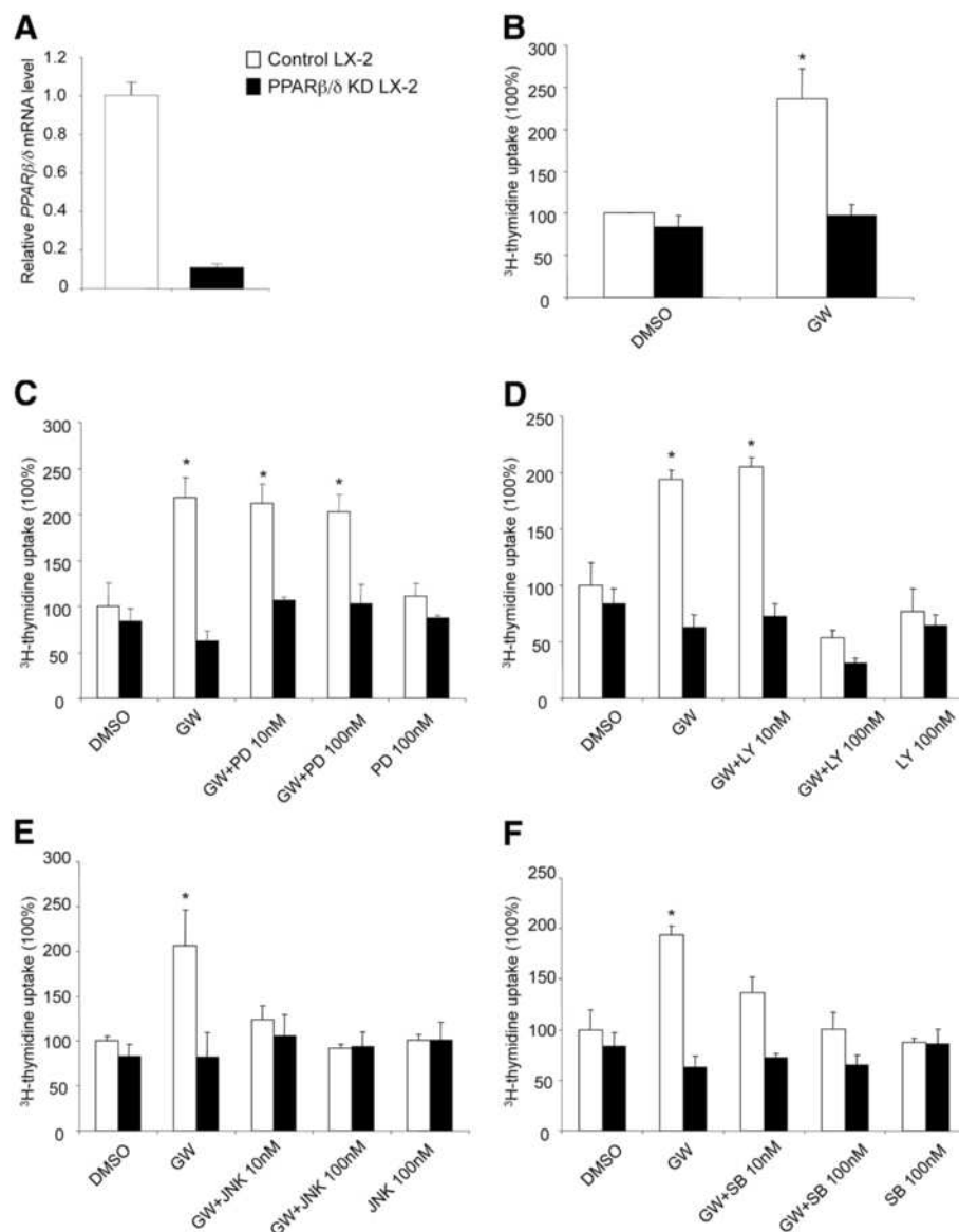
Figure 6 PPAR \beta/\delta controls pathways that regulate proliferation of LX-2 cells. Stable PPAR \beta/\delta knockdown (KD) was performed by lentiviral transduction of LX-2 cells with a siRNA against PPAR \beta/\delta . Control LX-2 cells were transduced with the control vector. A ) qRT-PCR showed reduced PPAR \beta/\delta expression in PPAR \beta/\delta KD LX-2 cells. The control values were set to 1. Results are means \pm SD of at least three independent experiments performed in triplicate. B-F ) Control and PPAR \beta/\delta KD LX-2 cells were starved for 24 h in serum-free media and then treated for 48 h with DMSO (control) or (B) 100 nM GW501516, or (C-F) 100 nM GW501516 in the presence or absence of 10 nM or 100 nM of (C) PD98059, (D) LY294002, (E) JNK inhibitor II, or (F) SB202190. All inhibitors were added 30 min before GW501516 treatment. Cell proliferation was determined by [ ^3\text{H} ]-thymidine incorporation. Values are expressed as a percentage of the values from DMSO-treated LX-2 cells, which were set to 100%. Values represent means \pm SEM from at least five independent experiments performed in triplicate; * = p < 0.05 compared to DMSO-treated cells.
