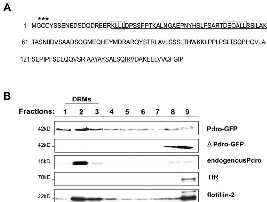
Figure 1. Identification and characterization of Pdro. (A) Full-length amino acid sequences of Pdro. Underlined amino acids indicate the position of peptide sequences determined by LC-MS/MS, boxes correspond to di-leucine motif (D/EXXXLL), stars indicate palmitoylation and myristoylation sites (C3 and 4 and G2 respectively). (B) DRMs from cells stably expressing Pdro-GFP (a c-terminus GFP-tagged protein) or \Delta Pdro-GFP (a c-terminus GFP-tagged mutant protein in which both Cys2 and 3 residues were substituted with Ala residues) were separated on a bottom-loaded sucrose step gradient. Probing the membrane with anti-GFP, anti-Pdro, anti-flotillin (DRMs marker) or anti-transferrin receptor (TfR, non-DRMs marker) antibodies assessed the distribution of proteins within fractions. Molecular-size standards (in kD) are shown on the left of the panel. The numbers represent the different fractions of the gradient. doi:10.1371/journal.pone.0010977.g001
