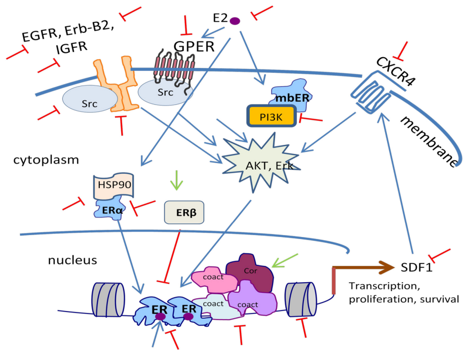
Schematic representation of some cytoplasmic, membrane and nuclear estrogen receptor (ER \alpha ) targets : estradiol (E2) activation of ER \alpha signaling is indicated by blue arrows; activation/enhancement of targetable proteins is indicated by green arrows, and inhibition with red T symbol.
