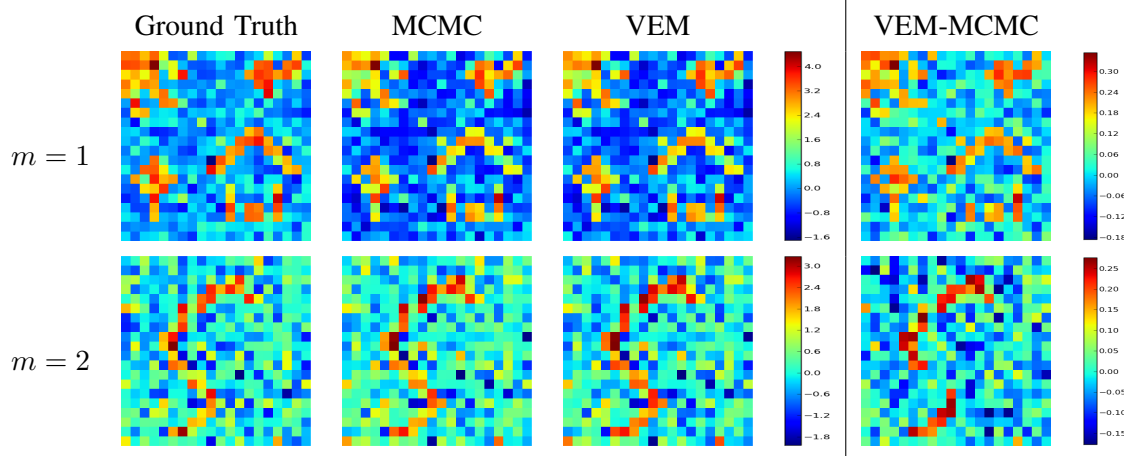
Fig. 5. Detection results for the first artificial data analysis. From left to right : Ground truth \alpha^m and NRL estimates \hat{\alpha}^m by MCMC and VEM, and NRL image difference ( \hat{\alpha}_{VEM}^m - \hat{\alpha}_{MCMC}^m ) ( right ). Top row: m = 1 ; bottom row: m = 2 .
