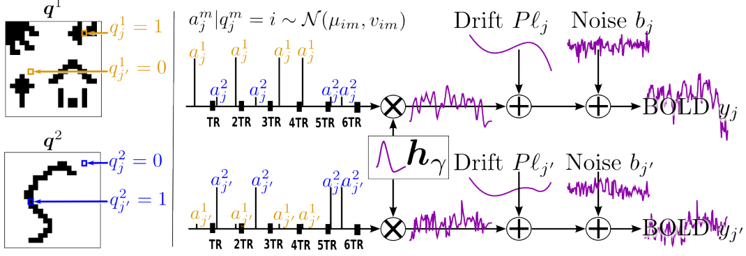
Fig. 2. Single parcel ( \mathcal{P}_\gamma ) artificial data generation process using two experimental conditions ( M = 2 ). From left to right : label maps q^m are hand-drawn. Conditionally on them, NRL values \{a_j^m, j \in \mathcal{P}_\gamma\} are drawn from Gaussian distributions with means \mu_{im} and variances v_{im} whenever q_j^m = i . Then, for any given voxel j , the stimulus sequence of a given experimental condition m is multiplied by the corresponding NRL value a_j^m . The resulting sequence is convolved with a normalized HRF h_\gamma which is common to all conditions and voxels. Nuisance signals are finally added (drift P l_j and noise b_j ) to form the artificial BOLD signal y_j .
