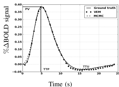
Fig. 6. Estimation results for the first artificial data analysis. Ground truth HRF h and HRF estimates \hat{h} using the MCMC and VEM algorithms.
