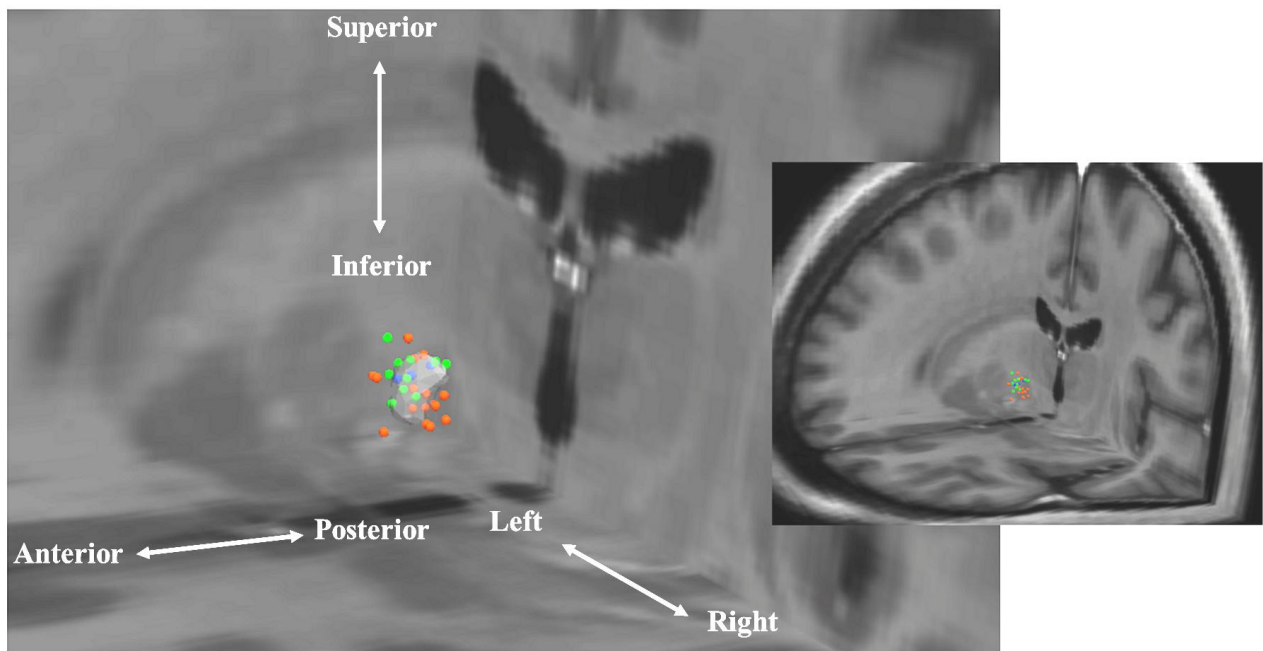
Fig. 3. UPDRS III analysis, with the cluster display in Talairach coordinates (above), and the cluster display in the template space for the left hemisphere with the STN (below).
