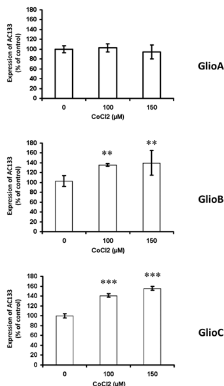
Figure 2. AC133 expression was up-regulated by CoCl 2 treatment in glioblastoma cells. Glioma cells, GliA, GliB, and GliC primary human glioblastoma cells cultured at 3% O 2 were incubated with 0, 100 and 150 μM CoCl 2 for 24 h and then analyzed for AC133 expression by flow cytometry. Results are expressed as percentage of control, representing the geomean fluorescence intensity levels obtained after immunostaining of AC133 for cells treated with vehicle alone. Results represent mean ± SEM of three independent experiments. Dunnett's test: **p<0.01, ***p<0.001.
