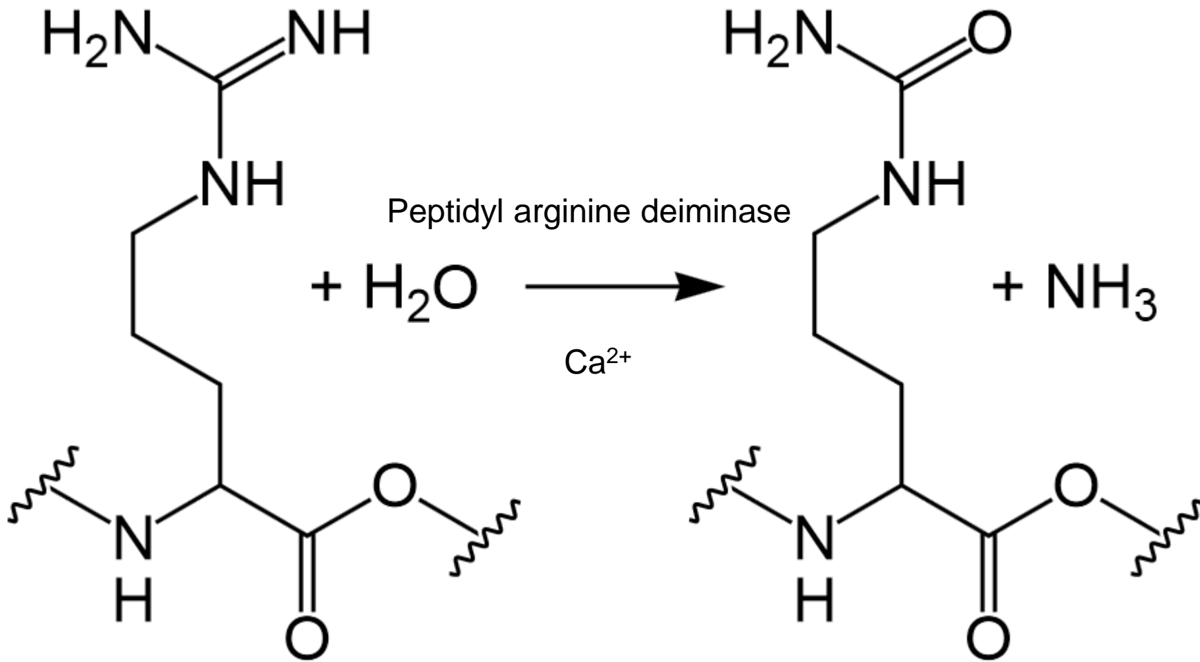
L-arginine (+charged)
