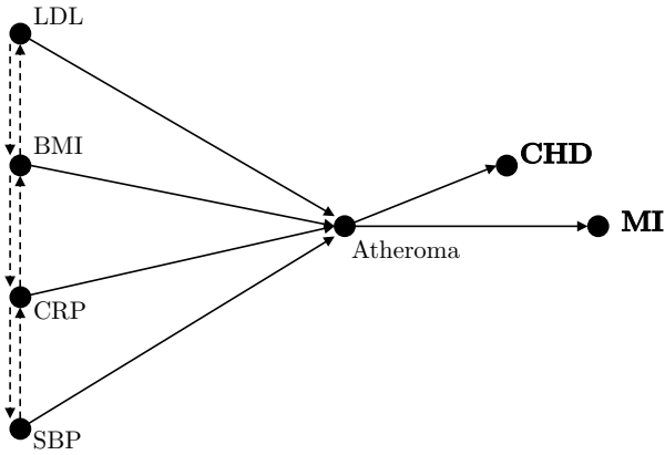
Fig. 2 Causal graph linking physiological conditions, atheromatous process, CHD and MI. Plain arrows mean purported causal influences and dashed arrows mean possible influences which have not been modeled in a mechanistic way and which result in correlations; we have not shown all the dashed arrows between LDL, BMI, CRP and SBP.
