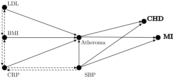
Fig. 3 Causal graph linking physiological conditions, atheromatous process, CHD and MI. Here SBP influences both the atheromatous process (effect on the drift) and directly CHD and MI (effect on the threshold). Plain arrows mean purported causal influences and dashed arrows mean possible influences which have not been modeled in a mechanistic way and which result in correlations; we have not shown all the dashed arrows between LDL, BMI, CRP and SBP.
