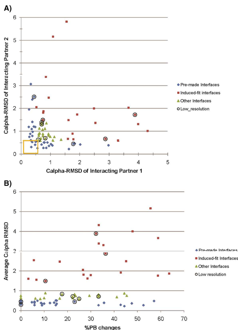
Figure 2 Characteristics of different types of interfaces. The three kinds of interfaces are pre-made (blue color), induced-fit (brown) and others (green). A). A plot of Cα RMSD for the pair of interacting partners is shown. Completely pre-made interfaces are enclosed in a yellow square. B). The extent of conformational change for the three kinds of interfaces is shown. The graphs plot only the majority of the points (Cα RMSD ≤ 6 Å) for the sake of clarity. This figure illustrates that A). Pre-made interfaces largely bind to induced-fit interfaces, and B). Although pre-made interfaces show small magnitude of structural change, the extent of conformational change they undergo is comparable to that observed in induced-fit/other interfaces. For both sets, points corresponding to complexes solved at a resolution >2.5 Å are encircled.
