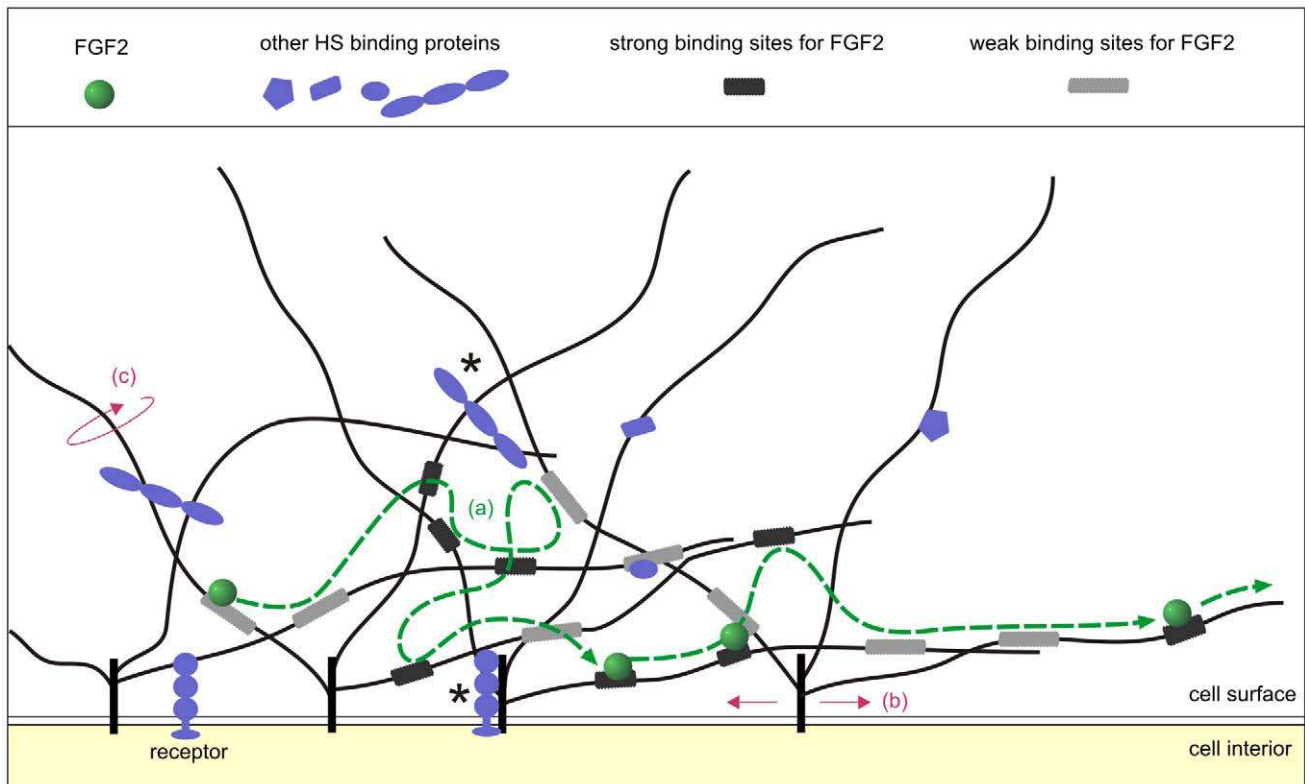
Figure 8. Schematic representation of the HSPG in the pericellular matrix. In the crowded pericellular matrix (macromolecular concentration of ~400 mg/mL), proteins and proteoglycans interact with each other. Only HSPG proteoglycans (in black and grey), the FGF2 (in green) and few other HS partners (in blue), are represented here for clarity. The HS-binding partners, which may be membrane-associated or “soluble” in the matrix, include growth factors, cytokines, chemokines, enzymes, matrix proteins, and numerous cell-surface receptors. Proteoglycan core proteins (black, inserted in the membrane) are shown with their HS chains (dark grey lines), which are between 40 to 160 nm long. Along these chains, dark grey rectangles represent stronger binding sites for FGF2, and light grey rectangles represent weaker binding sites for FGF2. These binding sites form non-random networks of heterogeneously distributed binding sites within which the FGF2 moves by translocating from one site to another (a). A path of the FGF2 is shown by green arrows and some of its successive positions marked as a green circle. This motion of the FGF2 is independent of the motion of the protein core of the HSPG itself (b). Movement of the HS chains (c) to which the FGF2 is attached may also contribute to the motion of the FGF2 within the pericellular matrix. Note that the many endogenous binding partners of HS chains and HSPG core proteins may, in some conditions, severely restrict the diffusion of the protein core and of the HS chains (asterisks). doi:10.1371/journal.pbio.1001361.g008
