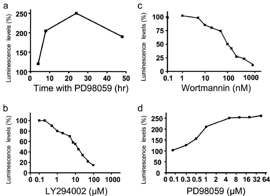
Figure 1 TF promoter activity in MDA-MB-231-TFluc cells treated by LY294002, wortmannin and PD98059. Panel a: MDA-MB-231-TFluc cells were treated by PD98059 at 10 μM for different time periods, then washed. Panels b-c: the cells were treated by LY294002 (b), wortmannin (c) and PD98059 (d) at indicated concentrations for 24 hrs. The activity of luciferase in the cells was measured. The data represent the means values of three independent experiments.
