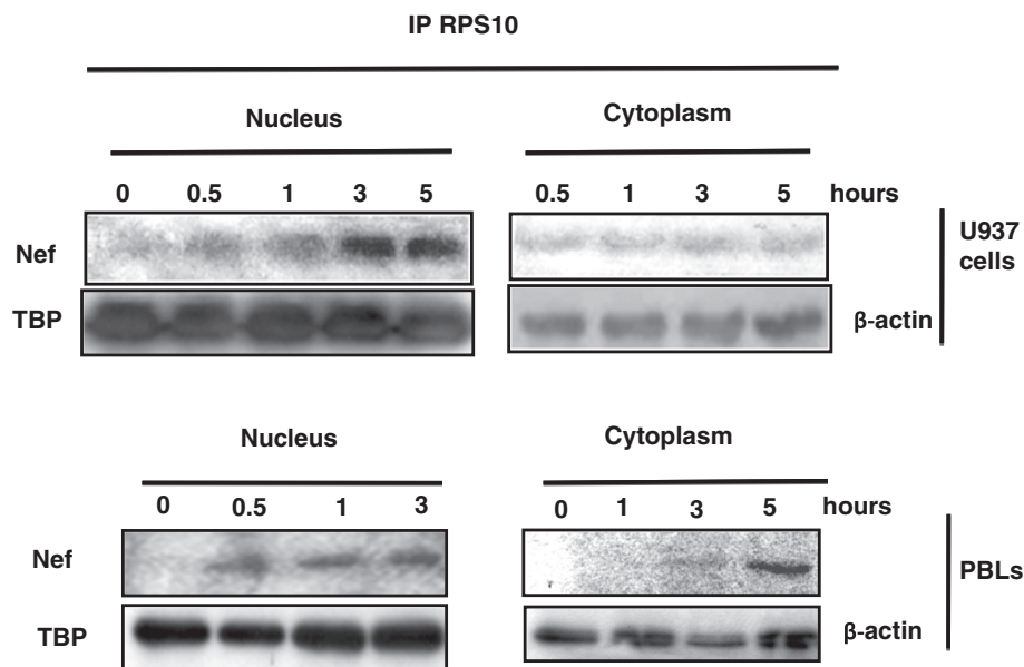
Figure 3 Time course of RPS10/rNef complexes in cells treated with rNef. Cytoplasmic and nuclear extracts from U937 cells and PBLs treated with rNef (100 ng/ml) for up to 5 hours were immunoprecipitated with an anti-RPS10 mAb. Immunoprecipitated material was analyzed by western blotting with an anti-Nef mAb. Results are representative of three independent experiments.
