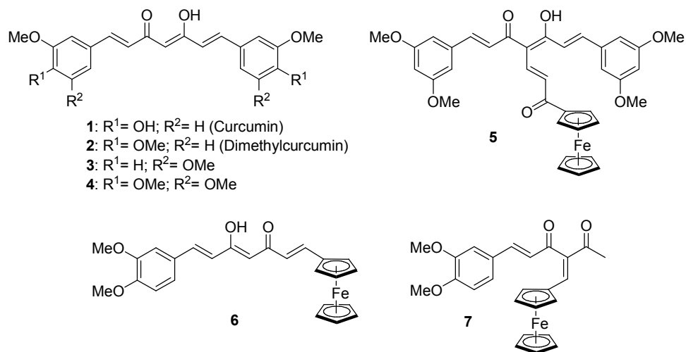
Figure 1. Organic curcuminoids and first ferrocenyl curcuminoid derivatives
