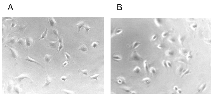
Figure 3. Morphological effects of the ferrocenyl curcuminoid 13 . Exponentially growing endothelial cells (EA.hy 926) were exposed to the solvent DMSO at 1% (panel A, control), or to the curcuminoid 13 at a concentration of 6.3 µM (panel B), and incubated for 2 h (37 °C, 5% CO 2 ). Representative photographs shown were recorded at an original magnification of 200 X.
