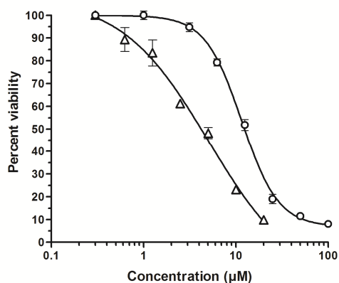
Figure 2. Percent viability of B16 melanoma cells as a function of the concentration of the organic 3,5-dimethoxycurcumin 3 (circles) or the ferrocenyl analogue 12 (triangles) (48 hour exposure time). Error bars, SD.
