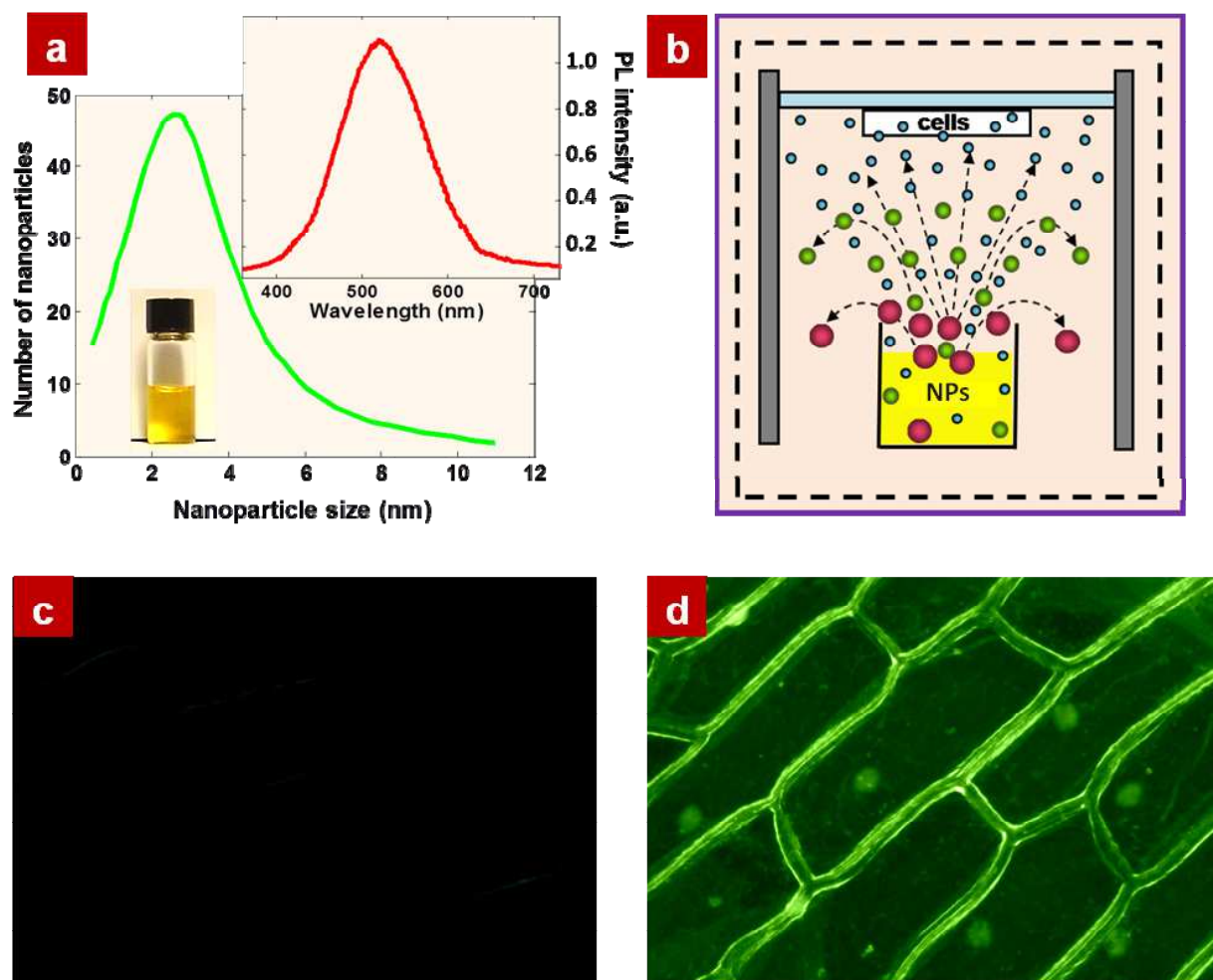
Figure 1 Size distribution of the NPs (a). Inset shows a typical photoluminescence spectrum of NPs obtained from 3 C-SiC. (b) Schematic view of the experimental set-up. Onion cells are mounted on a mobile holder situated above a colloidal suspension containing the fluorescent NPs. Fluorescence images of the onion epidermal cells exposed to the suspensions without (c) and with (d) NPs.
