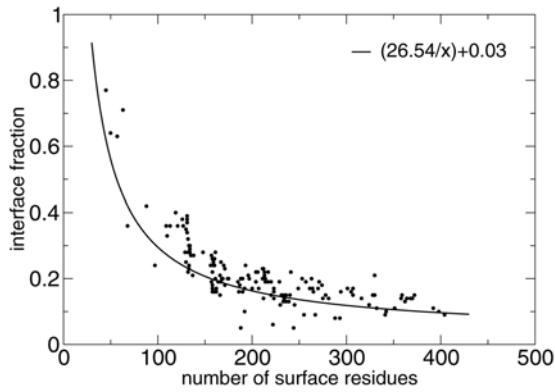
Figure 4. Protein surface size and interface fraction. Plot of the f_{\text{intfrac}} function relating surface size and fraction of the surface covered by the interface. Dots correspond to JET predictions on all proteins in the Huang dataset, where predicted interface sites are computed with mixed trace values. doi:10.1371/journal.pcbi.1000267.g004
