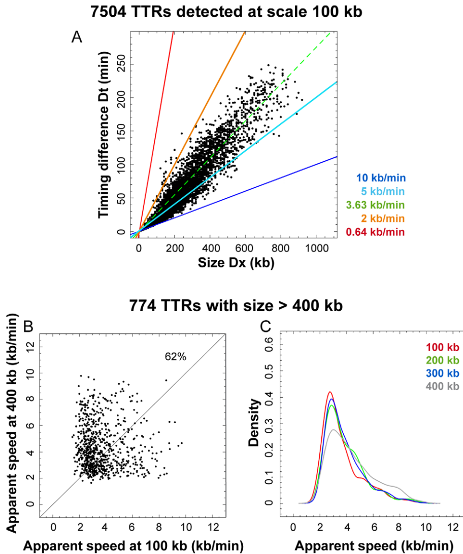
Figure 5. Replication Speeds along TTRs. (A) Size and replication time of individual TTR. The time difference, Dt , between the early and the late side of each TTR is plotted along its length, Dx , for each of the 7504 TTRs (open circles). By definition, the maximum replication speed of TTRs is 10 kb/min (dark blue line). The mean apparent replication speed, Dx/Dt , is 3.63 kb/min (green dashed line). The mean ( v = 2 kb/min, orange line) and maximum ( v = 0.64 kb/min, red line) velocities of single forks measured by DNA combing are indicated. Only 24 TTRs lie between the orange line and the vertical axis. (B) Evolution of apparent replication speed along the 774 TTRs > 400 kb. The apparent speed measured at the distance D_4 = 400 kb from early edge of each TTR is plotted against the apparent speed measured at the distance D_1 = 100 kb. Replication accelerates for 62% of TTRs. (C) Distribution of apparent replication speeds along the 774 TTRs > 400 kb. The apparent speed has been measured at different distances D_1 – D_4 from early edge of each TTR: D_1 = 100 kb, red curve; D_2 = 200 kb, green curve; D_3 = 300 kb, blue curve; D_4 = 400 kb, grey curve.
