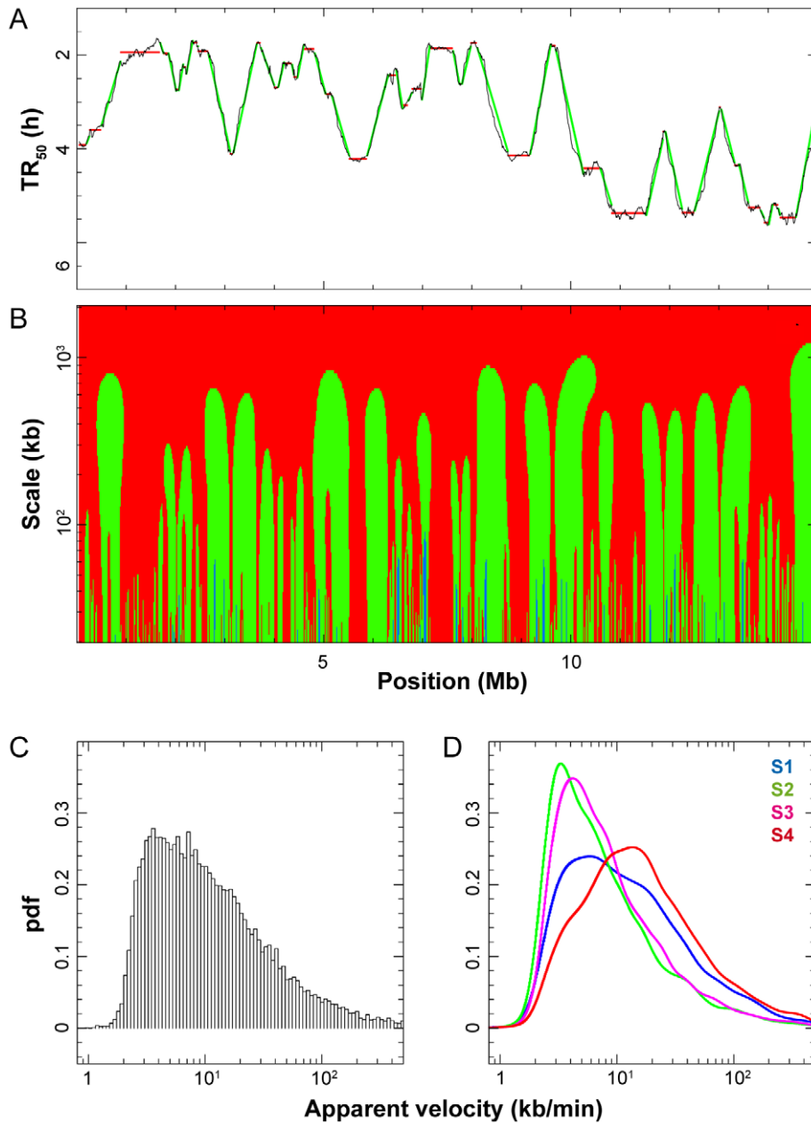
Figure 3. Replication timing profiles segmented in CTRs/TTRs and multiscale analysis of apparent replication speeds in HeLa cells. (A) Profile of replication timing ( TR_{50} , hours) along a 15 Mb segment of chromosome 17. Small TR_{50} values correspond to early replicating regions; large TR_{50} values correspond to late replicating regions. The replication timing profile was segmented into regions that replicate at apparent speed >10 kb/min (CTRs: Constant Timing Regions, red horizontal lines) and <10 kb/min (TTRs: Timing Transition Regions, green oblique lines) at scale 100 kb. (B) Multiscale analysis of apparent replication speeds along the same chromosome segment. Replication speeds determined by wavelet transform analysis (see Material and Methods) at scales indicated on the y-axis are shown in three colors (blue, <2 kb/min; green, from 2 to 10 kb/min; red, >10 kb/min). (C) Distribution of apparent replication speed at the 100 kb scale in the whole genome (pdf: probability density function). (D) Distribution of apparent replication speeds in the four temporal compartments of S phase: S1, S2, S3 and S4 (respectively: blue, green, pink, and red curves). doi:10.1371/journal.pcbi.1002322.g003
