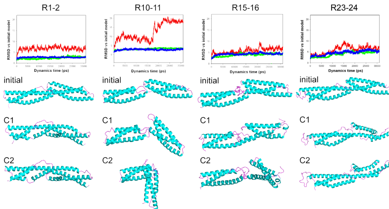
Figure 4. Structural changes in the four tandem repeats observed during the molecular dynamics relaxation. \text{C}\alpha RMSD measured between the initial models and snapshots of the four molecules taken every ps. The red line represents the RMSD of the tandem repeats, the green indicates the RMSD of the N-terminal repeat in the tandem and the blue shows the RMSD of the C-terminal repeat. The simulations were submitted to a clustering procedure in order to identify two clusters per simulation. \text{C}\alpha backbone traces of the initial model and the snapshots closest to the center of each cluster (C1 and C2) are shown with the same orientation as in Fig. 1B. doi:10.1371/journal.pone.0023819.g004
