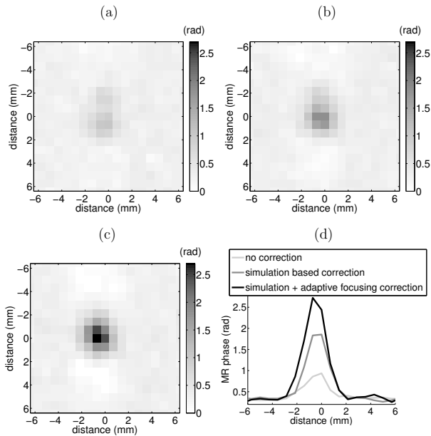
FIG. 9. MR-ARFI encoded displacement obtained with: (a) no correction, (b) simulation based correction alone, (c) simulation based correction plus energy-based adaptive focusing correction. (d) Lateral profiles of the slices.
