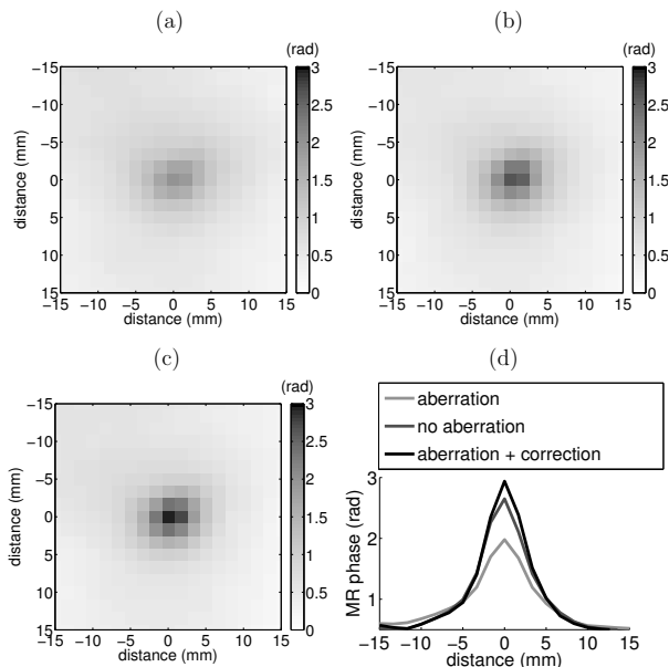
FIG. 7. MR-ARFI encoded displacement obtained with: (a) aberration, (b) no aberration, (c) aberration and energy-based adaptive focusing correction. (d) Lateral profiles of the slices.
