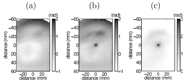
FIG. 2. (a) MR-ARFI phase image without US emission, (b) with US emission. (c) Final encoded displacement given by the difference of both images.
