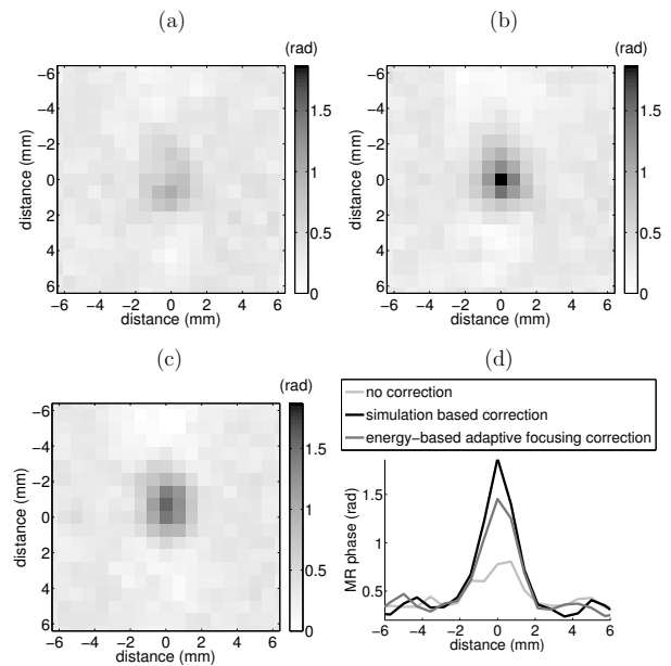
FIG. 8. MR-ARFI encoded displacement obtained with: (a) no correction, (b) simulation based correction, (c) energy-based adaptive focusing correction. (d) Lateral profiles of the slices.
