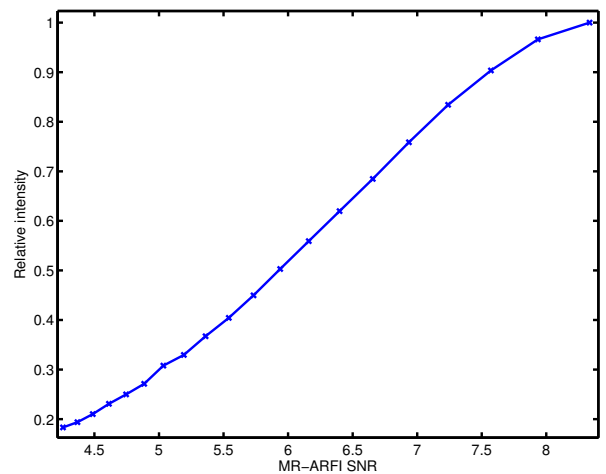
FIG. 10. Estimated acoustic intensity relative to the optimal focusing intensity.
