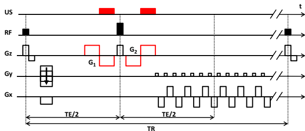
FIG. 1. MR-ARFI sequence used for the adaptive focusing of HIFU beams. Two rectangular bipolar MSG were added to a standard multislice spin-echo sequence with EPI readout. Two sonications were synchronized to the MSG periods.
