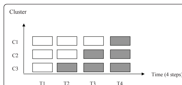
Figure 1 Design of the CONFUCIUS study. One cluster (C1, C2 or C3) represents one surgical ward. One unit (control or intervention) represents one time period of one cluster. "White square": "control" unit = surgical wards without multifaceted prevention program "Black square": "intervention" unit = surgical wards with multifaceted prevention program.
