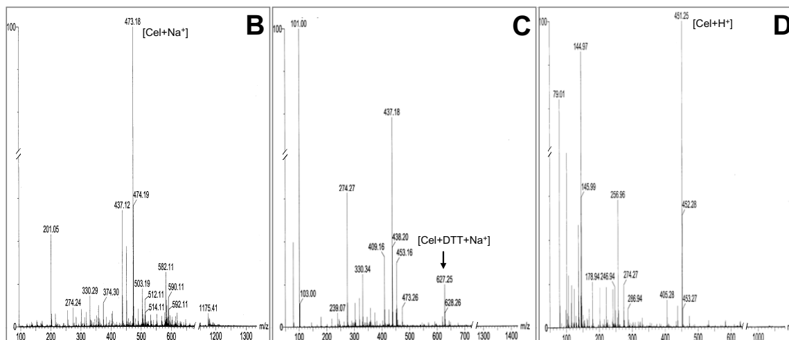
Figure 6 Reactions between celastrol and thiol-containing agents and between celastrol and non-thiol small molecules. A: Absorption spectra of celastrol mixed with different agents. Celastrol was mixed with different small molecules in ratio of 1:2, the absorption spectra then detected. B-D: Mass spectrum analysis of the following agents or reactions: (B) celastrol; (C) the mixture of celastrol and DTT at a 1:2 molar ratio in DMSO; (D) celastrol and DTT reaction result with formic acid added (to save space, the detection patterns presented have been truncated. The non-truncated view can be found in this manuscript's additional file 2).
