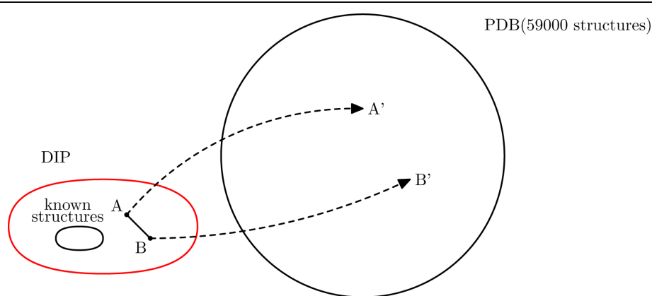
Figure 1 Benchmark generation. For each interacting pair of proteins with unknown structure, we use a proxy pair of homologs with known structure.
