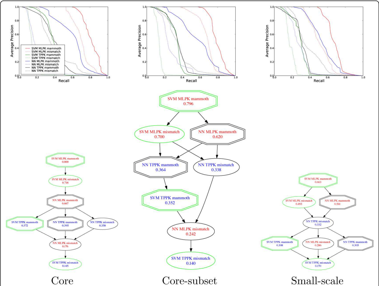
Figure 2 Comparison of methods for predicting protein-protein interactions. The top three panels plot the average precision (TP/(TP+FP)) as a function of recall (TP/(TP+FN)) for the core, core subset and small-scale benchmarks. Each precision is averaged across the 15 splits of 3x5cv, and estimated for test sets for which the negative examples are not downsampled. In the lower three panels, an edge from method A to B indicates that method A outperforms method B at p > 0.5 according to a Wilcoxon signed rank test applied to the area under the precision-recall curve, computed separately for each of the 15 splits of 3x5cv. Redundant edges have been removed for clarity; i.e., the figure shows the transitive reduction of the full graph.
