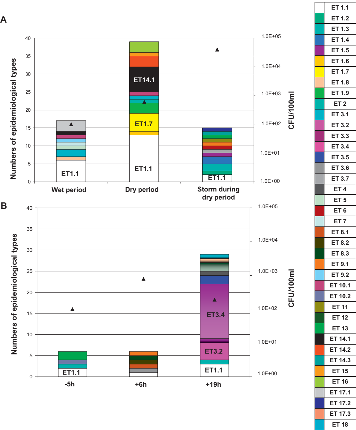
Figure 3 Distribution of E. coli B1 epidemiological types in relation to hydrological conditions (A) and before and after a rain event during a wet period (B).
