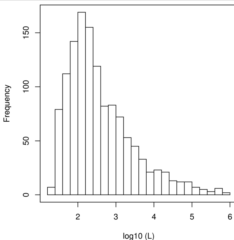
Figure 4 Histogram of the \log_{10}(L) for 1,276 PROSITE patterns in the framework of an order 1 Markov model. Note that the 0.1% patterns with the largest complexities have been removed from the graph in order to improve readability.
