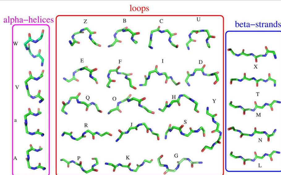
Figure 2 Geometry of the 27 structural letters of the HMM-27 structural alphabet.
