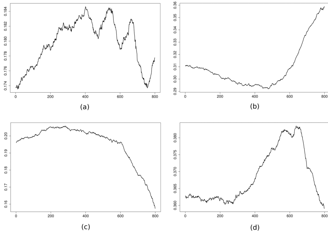
Figure 5 Some transitions of the order 1 heterogeneous Markov model fitted using a sliding window of size 200 on the upstream region data set. The plots respectively correspond to the following quantities: a) \pi_i(A, G) ; b) \pi_i(G, A) ; c) \pi_i(G, G) ; d) \pi_i(T, T) , 1 \leq i \leq 800 .
