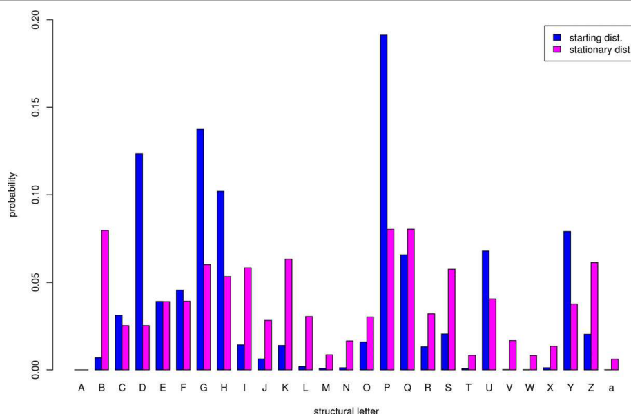
Figure 3 Starting and stationary distributions of the 27 structural letters in the loop structure data set.
