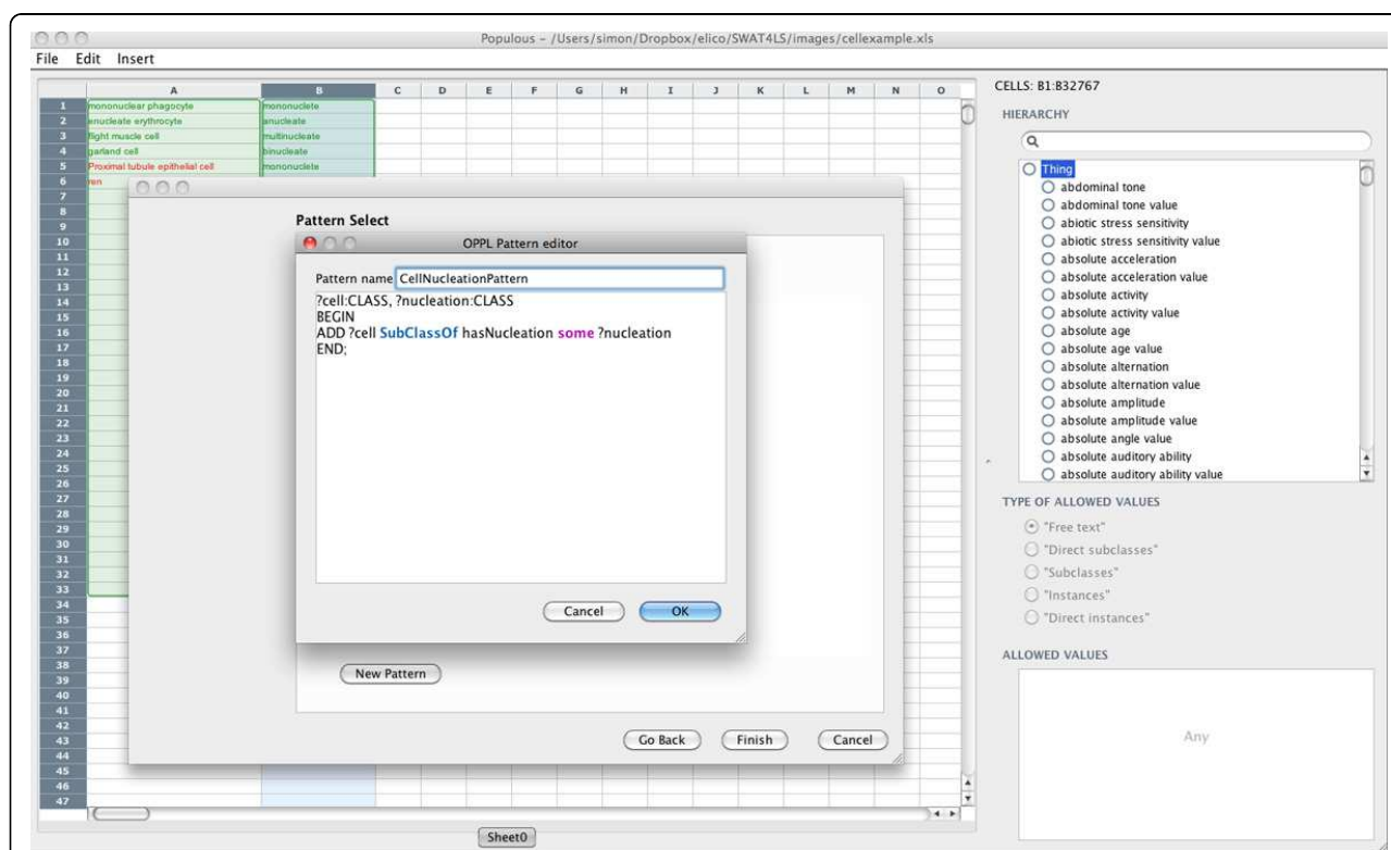
Figure 5 Populous OPPL wizard. Screenshot of Populous Pattern Wizard showing the OPPL script editor.
