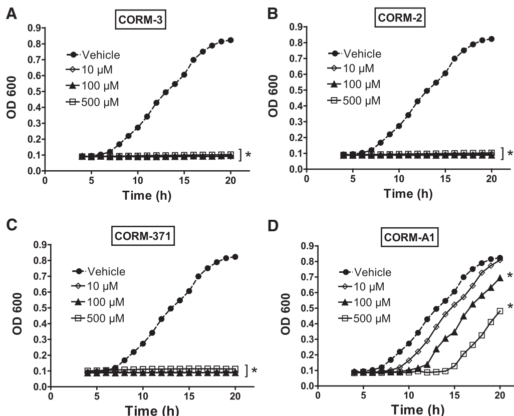
FIG. 3. Effect of CO-RMs on Pseudomonas aeruginosa growth. Bacterial growth was followed for 20 h after treatment with CO-RMs (10, 100 and 500 μM) or vehicle and was assessed by measuring spectrophotometrically the optical density at 600 nm. The initial PAO1 inoculum was 4 \times 10^6 cfu/ml. The vehicle used was sodium chloride 0.9% for the water-soluble CORM-3 (A), CORM-371 (C), and CORM-A1 (D) and 0.1% DMSO for the lipid soluble CORM-2 (B). Curves represent means of 6 independent experiments; error bars are omitted for clarity. * p < 0.05 versus vehicle. DMSO, dimethyl sulfoxide; PAO1, Pseudomonas aeruginosa .
