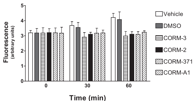
FIG. 5. Production of H 2 O 2 in PAO1 bacteria treated with CO-RMs. The production of H 2 O 2 in bacteria treated with 100 \mu\text{M} CORM-2, CORM-3, CORM-371, or CORM-A1 was measured fluorometrically after addition of 2'-7'-dichlorodihydrofluorescein diacetate (see Materials and Methods for details). Sodium chloride 0.9% (vehicle) and DMSO were used as negative control for CORM-3 and CORM-2, respectively. Each bar represents the mean \pm SEM of six independent experiments. H 2 O 2 , hydrogen peroxide.
