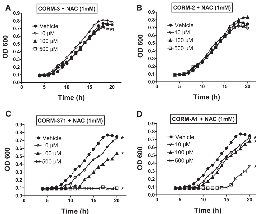
FIG. 6. Effect of CO-RMs on PAO1 growth in the presence of NAC. Bacterial growth was followed for 20 h after treatment with CO-RMs (10, 100 and 500 \mu M) or vehicle in the presence of 1 mM NAC and was assessed by measuring spectrophotometrically the optical density at 600 nm. Initial PAO1 inoculum was 4 \times 10^6 cfu/ml. The vehicle used was sodium chloride 0.9% for the water-soluble CORM-3 (A), CORM-371 (C), and CORM-A1 (D) and 0.1% DMSO for the lipid soluble CORM-2 (B). Curves represent means of six independent experiments; error bars are omitted for clarity. * p < 0.05 versus vehicle. NAC, N-acetylcysteine.
