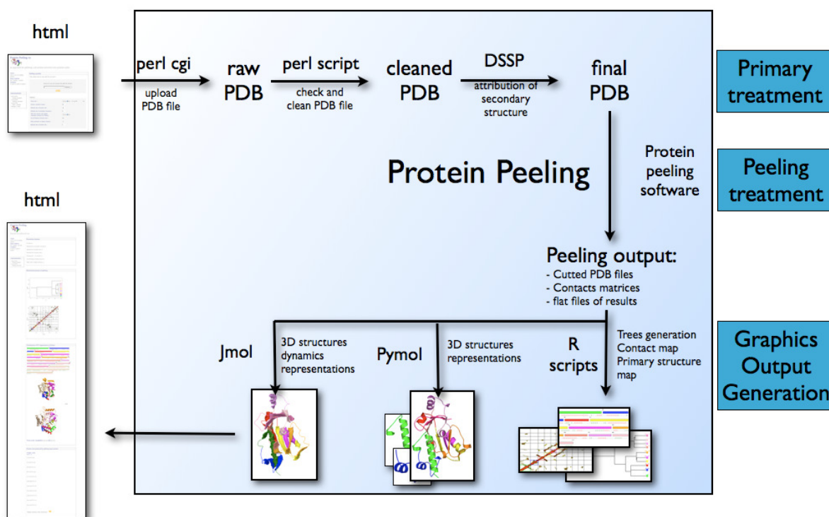
Figure 2. Principle of PP2 web server. All the different steps of the process are presented with the actions done and the language / software.
