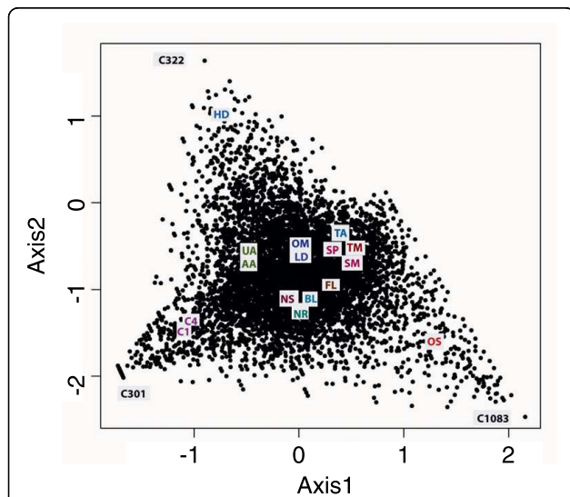
Figure 5 Principle component analysis of all the libraries based on frequencies of expression across all 16 different conditions. The plot shows the axes with maximum variation. For two-letter library codes, see Table 1.
