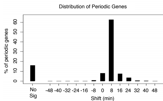
Figure 3 Distribution of periodic genes identified by Orlando et al. in (Orlando et al. 2008). Each of the 1274 periodic genes identified by Orlando et al. was assigned to its maximally significant shift. Genes which did not have a significant p-value (< 0.001) were assigned to the "Not Significant" category.
