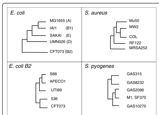
Figure 1 Neighbor joining trees based on genomic MUMi distances of the strains selected for the five-genome alignments.
