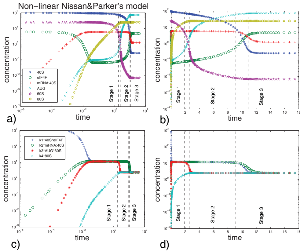
Figure 5 Simulation of the non-linear protein translation model. Simulation of the non-linear protein translation model with parameters k_1 = 2 , k_2 = 2 , k_3 = 5 , k_4 = 0.1 , [40S]_0 = 100 , [60S]_0 = 25 , [eIF4F]_0 = 6 . a) and b) chemical species concentrations at logarithmic and linear scales; c) and d) reaction fluxes at logarithmic and linear scales. By the dashed line several stages are delimited during which the dynamics can be considered as (pseudo-)linear. To determine where “>>” and “<<” conditions are violated, we arbitrarily consider “much bigger” or “much smaller” as difference in one order of magnitude (by factor 10).
