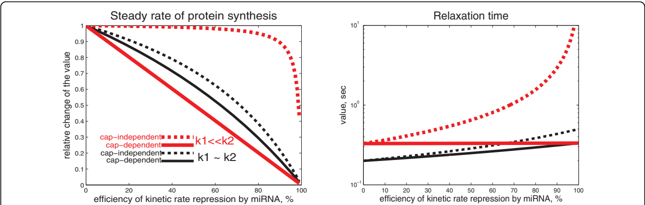
Figure 3 Predicted change in the steady-state rate of protein synthesis and its relaxation time. Graphs illustrating the predicted change in the steady-state rate of protein synthesis (left), and its relaxation time, i.e., the time needed to recover from a perturbation to the steady state value (right). Four curves are presented. The black ones are for the wild-type cap structure, which is modeled by k_1 = k_2 . The red ones are for the modified structure, when k_1 \ll k_2 . The main conclusion from the left graph is that if microRNA acts on a late initiation step, diminishing k_2 , then its effect is not measurable unless k_2 is very strongly suppressed (as reported in [41]). The main conclusion from the right graph is that the effect of microRNA can be measurable in this case if one looks at dynamical features such the relaxation time.
