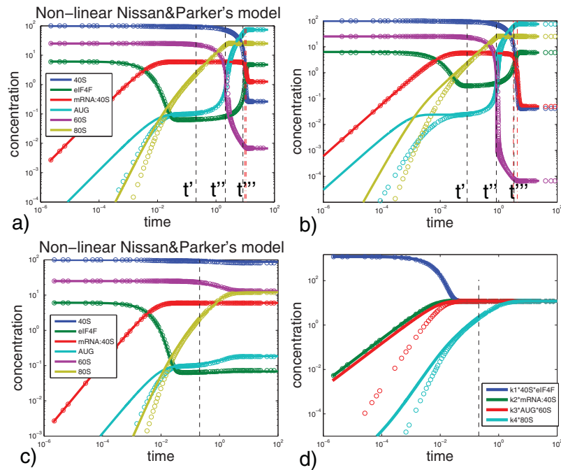
Figure 7 Comparison of the numerical and approximate analytical solutions of the non-linear protein translation model. Examples of the exact numerical (circles) and approximate analytical (solid lines) solutions of the non-linear protein translation model. a) For the set of parameters k_1 = 2, k_2 = 2, k_3 = 5, k_4 = 0.1 ; b) For parameters k_1 = 1, k_2 = 5, k_3 = 50, k_4 = 0.01 ; c) For the set of parameters from [41], k_1 = 2, k_2 = 2, k_3 = 5, k_4 = 1 ; d) Reaction fluxes for the set of parameters c). Dashed black vertical lines denote evaluated transition points between the dynamics stages. Dashed red vertical points denote the time points where [40S](t) = 10[eIF4F](t) and [40S](t) = [eIF4F](t)/10 respectively.
