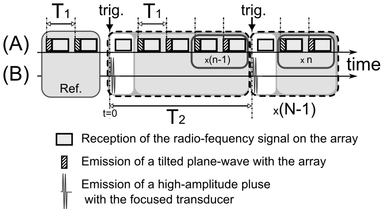
Figure 3: The nucleation detection sequence. The two time lines represent the timing sequence for (A) the ultrasound scanner driving the linear array and, (B) the high power channel driving the single-element transducer. The synchronization of the time lines occurs at t=0 with the triggering event (trig.). The blocks “synchronized high-amplitude emission and passive detection” are marked by the white rectangle including the triggering event, and the
