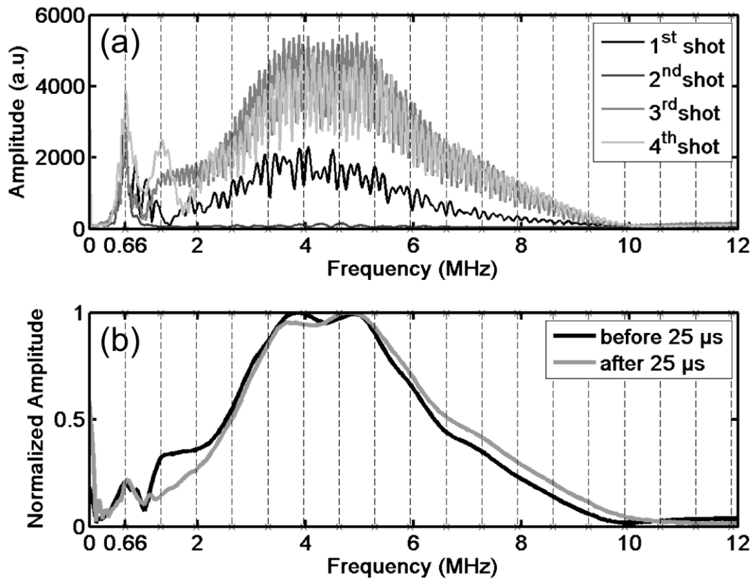
Figure 6: (Gelatin gel) Magnitude of the Fourier transform of the unfiltered passive radio-frequency data for (a) all of the different shots and the whole duration of the recorded signals, (b) the third shot analyzed in two separate parts: before and after 25 \mu\text{s} from the beginning of passive recording. The spectral traces shown are averages over the 64 channels. For (b), the spectral traces are normalized to their maximum. The vertical dashed lines indicate the integer multiples of the central frequency of the high-amplitude excitation pulse (660 kHz).
