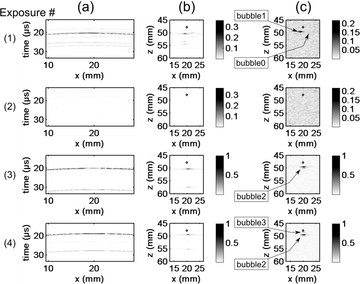
Figure 4: (Gelatin gel) Images of the different detection acquisitions for the first four high-amplitude exposures. Each line corresponds to a different shot: (a) high-pass filtered passive radio-frequency data, (b) the corresponding passive beamformed image, (c) the second active
