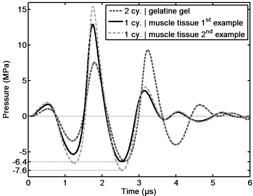
Figure 2: Pressure waveforms of the therapy pulse at the focal point of the therapy transducer. The signals shown are the averages of 15 acquisitions low-pass filtered below 50 MHz (FIR, Butterworth high-pass digital filter design, order 3, 50 MHz cutoff frequency). Each waveform corresponds to a different excitation used in this paper: a two-cycle excitation for the gelatine gel, and two different one-cycle excitations for the muscle samples. The measurements were recorded in degassed water. The peak negative pressure is indicated on the pressure axis.
