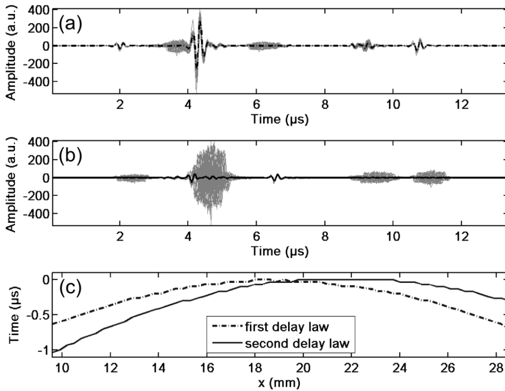
Figure 7: (Gelatin gel) Alignment of the filtered passive radio-frequency (RF) data for the first shot, (a) and (b) display the alignment of the RF data corresponding to the first and second time delay laws plotted in (c), respectively. For (a) and (b), the superimposed gray curves are the 64 delayed passive signals received on the elements of the ultrasonic array, and the thick line shows their averages.
