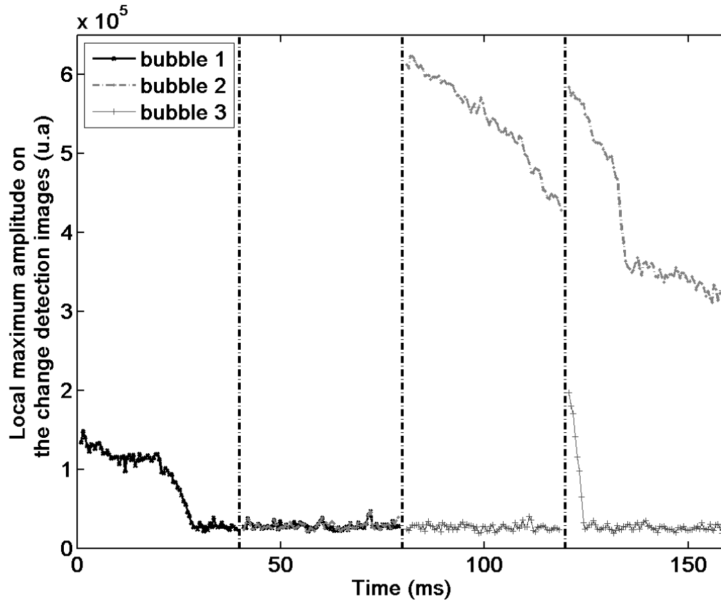
Figure 5: (Gelatin gel) Evolution of the scattering amplitude of the cavitating regions identified in Figure 4. The vertical dash dotted lines indicate the high-amplitude shots.
