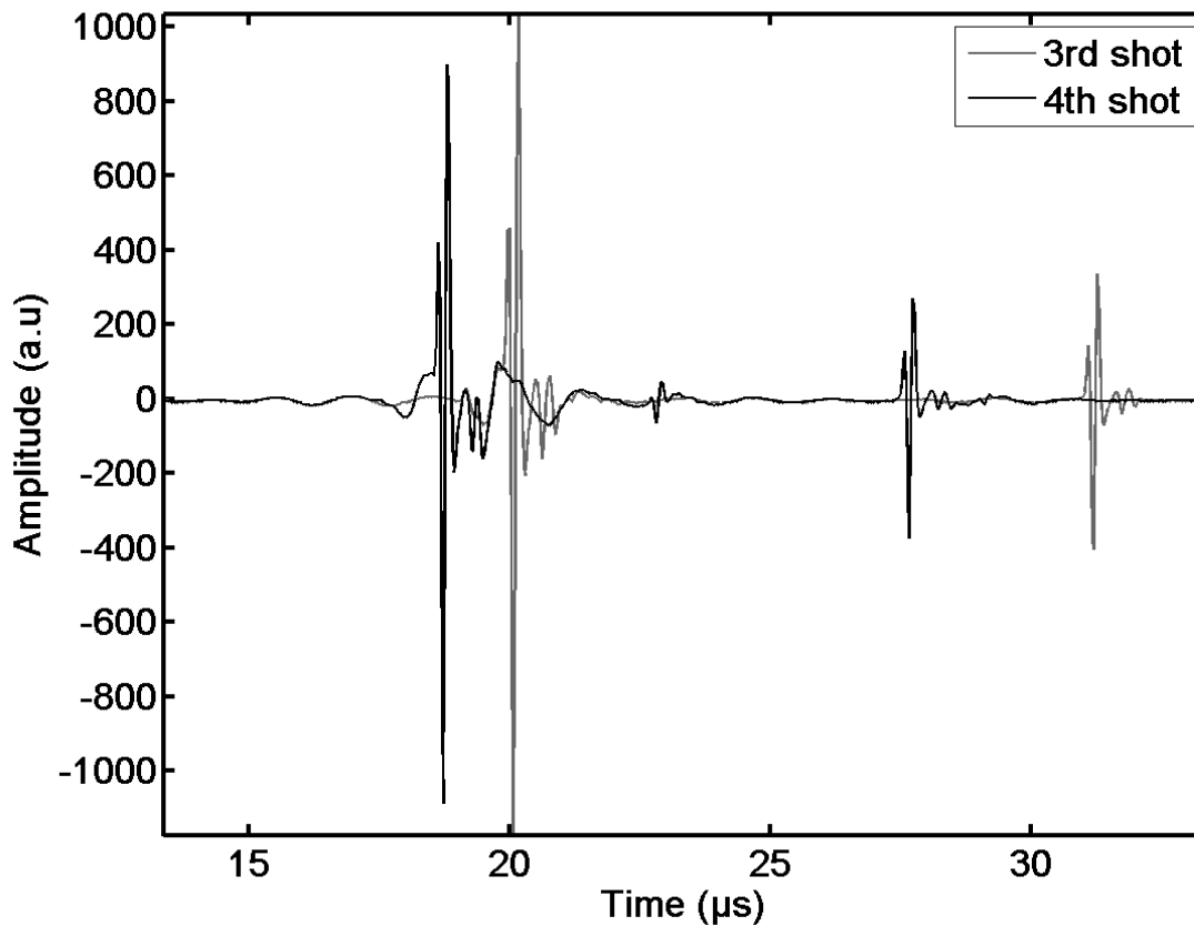
Figure 8: (Gelatin gel) Unfiltered passive radio-frequency signals recorded with the 65 th element of the array for the third and fourth shots.
