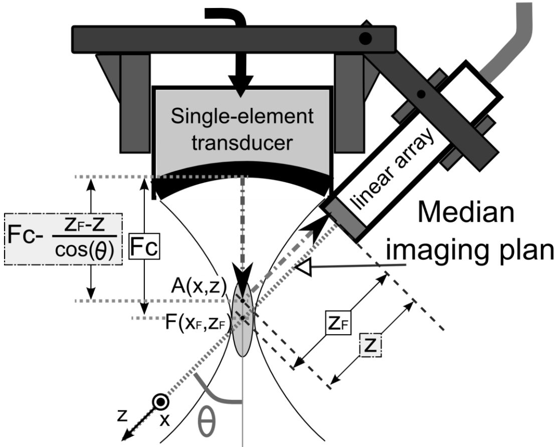
Figure 14: Diagram of the synchronized passive beamforming
