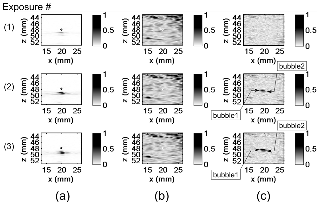
Figure 10: (First sheep thigh muscle sample) Images of the different detection acquisitions for the first three high-amplitude exposures. Each row corresponds to a different shot: (a) the beamformed image corresponding to the high-pass filtered passive radio-frequency (RF) data, (b) second raw RF active image for each shot, and (c) the corresponding change detection image. The x axis origin is set to the first element of the array. For columns (b) and (c), the focus point of the single-element transducer is marked with a white rhombus ( z=47.9 mm, x=19.8 mm). The beamformed data are normalized to the brightest point of the series for (b) and (c).
