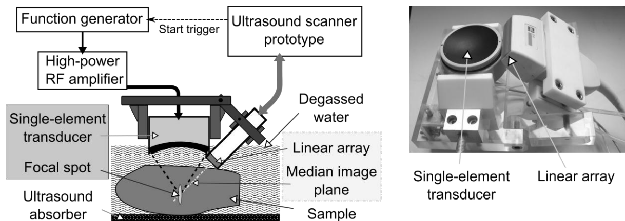
Figure 1: Experimental set-up. Drawing (a) represents a schematic side view of the integrated high-amplitude focused ultrasound and imaging system and a schematic diagram of the driving electronics. The interrogation path (-.-) of the linear array is coaxial with the single element transducer focal spot. Picture (b) shows the integrated system.
