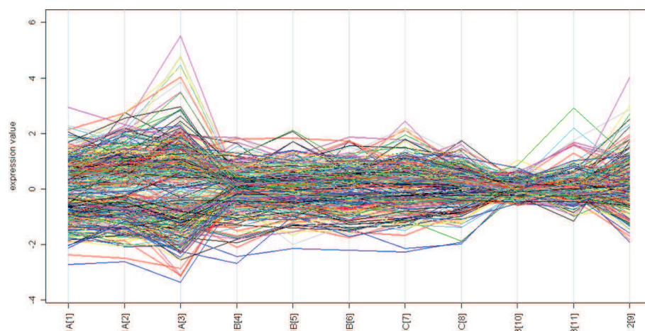
Figure 2 Magnitude of fold change expression characterizing E. coli , S. aureus , and S. uberis infections in cattle. The x-axis shows the time points {from 1 to 11} of each different cattle experiment (1A, 1B, 1C, 2, and 3; Table 2), while the y-axis shows the fold changes for each gene (each line). High differences are observed especially during infection with E. coli (1A {3}), and to a lesser extent with S. uberis (2 {9}).
