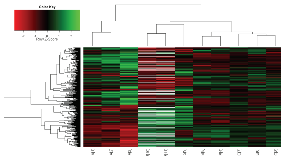
Figure 1 Heat map showing cluster analysis of the microarray experiments used in the cattle-specific response to three different pathogens ( E. coli , S. aureus , and S. uberis ). The x-axis shows the time points {from 1 to 11} of each different cattle experiment (1A, 1B, 1C, 2, and 3; Table 2), while the y-axis displays the clustered genes. The map itself contains gene fold changes Z-score normalized over all time points. They are color coded, with red corresponding to down-regulation and green to up-regulation. White lines in experiment 3 represent missing genes not present on the microarray. The first clustering step is primarily based on experiment number (Tables 1 and 2) (experiment 1A {1-3} clustered together, 1B {4-5} clustered together, 1C {7-8} clustered together along with the 1B time point {6}, and 3 {10-11} clustered together). The final clustering steps indicated a pathogen-specific pattern as all S. aureus time points (along with the S. uberis time point {9}) clustered together, separately from the E. coli time points.
