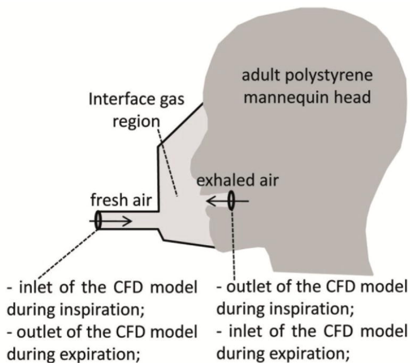
Schematic of the set-up showing the interface positioned on the polystyrene mannequin head. CFD: Computational fluid dynamics
