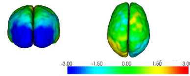
Fig. 5. Asymmetry maps obtained for one of the SI subject. We display the same views and the same components as in Figure 4. From left to right: left-right, head-foot, posterior-anterior components of the asymmetry field.
