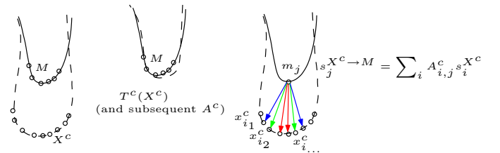
Fig. 2. Projection of scalar information on the mean shape: From left to right i) mean shape M and X^c . ii) M and T^c(X^c) (computed jointly with M ). iii) the subsequent correspondences (hot (resp. cold) colors indicate high (resp. low) values for A_{i,j}^c ) between each point m_j and points of X^c allow to compute the projected scalar information at point m_j of M .
