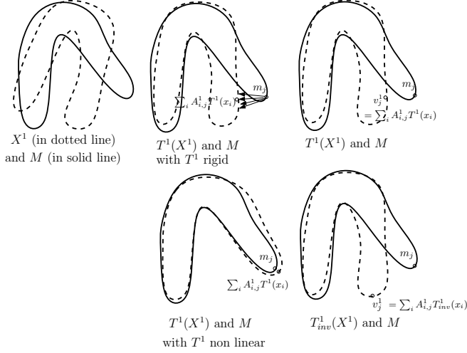
Fig. 1. First row: Illustration of the classical MS-EM-ICP (MS1). From left to right: i) the point set X^1 and M , ii) T(X^1) and M ( T^1 is a rigid-body transformation) and the resulting matching \sum_i A_{i,j}^1 T^1(x_i) and iii) the resulting correspondences v_j^1 = \sum_i A_{i,j}^1 T^1(x_i) , Second row: Illustration of the improved MS-EM-ICP (MS3). From left to right: i) T^1(X^1) on M ( T^1 is a non-linear smooth transformation) and the resulting matching \sum_i A_{i,j}^1 T^1(x_i) and ii) the resulting correspondences v_j^1 = \sum_i A_{i,j}^1 T_{inv}^1(x_i) .
