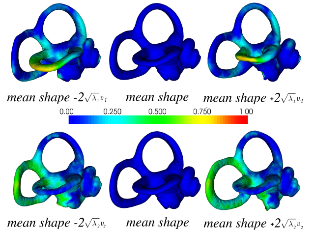
Fig. 3. Mean shape and first modes of variation on 15 osseous labyrinths. The magnitude of the deformations around the mean are mapped. The first mode of variation can be mainly interpreted as a change of size and of position of the lateral semicircular canal. The second mode of variation can be mainly interpreted as a change of size of the posterior semicircular canal.
