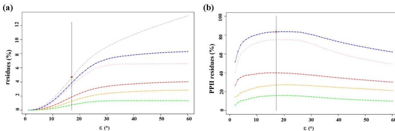
Figure 2. Deriving PPII assignment criterion: Choice of epsilon. (a) shows the percentage of residues found for \varepsilon ranging from 0 to 60^\circ . The percentage of amino acids associated to DSSP coil is shown in grey, PII assigned by PROSS is indicated in pink, assignment by XTLSSTR is in red and that of SEGNO in orange. In blue is shown the percentage of residues considered as PPII at least by one of the three SSAMs and the green plot indicates percentage of common assignments. (b) The same information is given as the percentage of PPII residues (in regards to DSSP coil). In the initial search, the epsilon chosen corresponds to 17^\circ , it is indicated by a black line.
