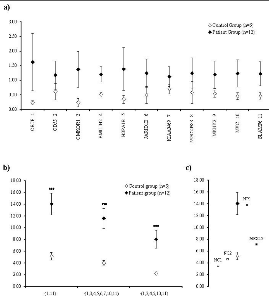
Figure 1 Weighted accumulative permutation analysis for differentiation between groups (WAPDG) results. (a) Means of the 1,000-fold permuted expression values per gene in patients and controls. (b) Results of summarised analysis including different subsets of genes. (c) Results of WAPDG analysis of two novel patients (NP1 and MRX13) and two novel controls (NC1 and NC2). The error bars represent the SD.
