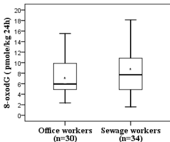
Figure 3 Box and whisker plot for the 24 hours urinary 8-oxodG level (pmole/kg 24 hours) in sewage and office workers, P = 0.28 for the mean differences. * Mean 8-oxodG, 8-oxo-2'-deoxyguanosine.
