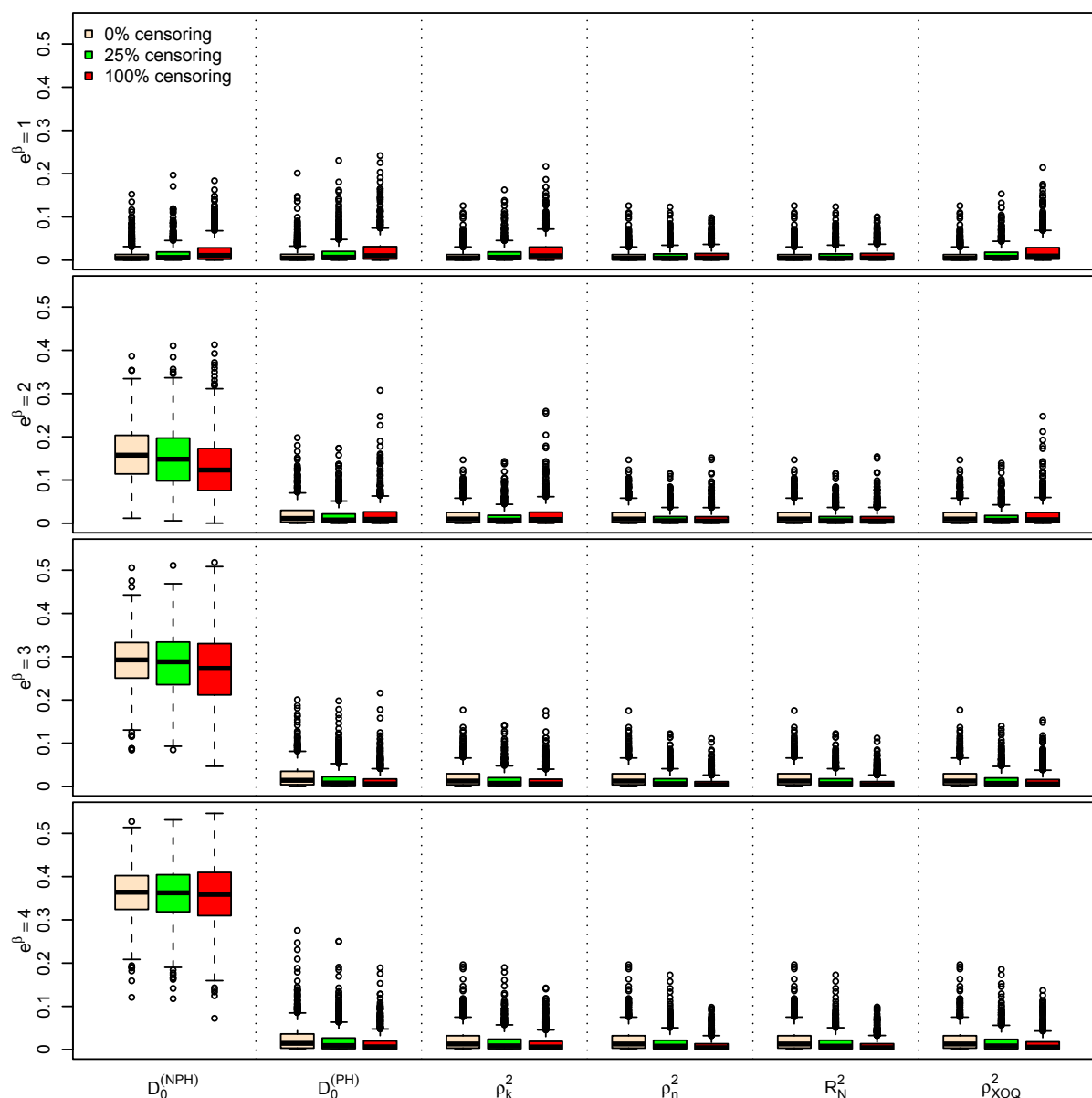
Figure 1 Simulations results for D_0^{(\text{NPH})} , D_0^{(\text{PH})} , \rho_N^2 , \rho_k^2 , R_N^2 and \rho_{\text{XOQ}}^2 , for n = 100 subjects, Z \sim \mathcal{B}(1/2) , X \sim \mathcal{W}(1, e^{\beta Z}) and a uniform censoring (1,000 repetitions). Boxplots of the different indices according to the values of e^\beta and p_c .
