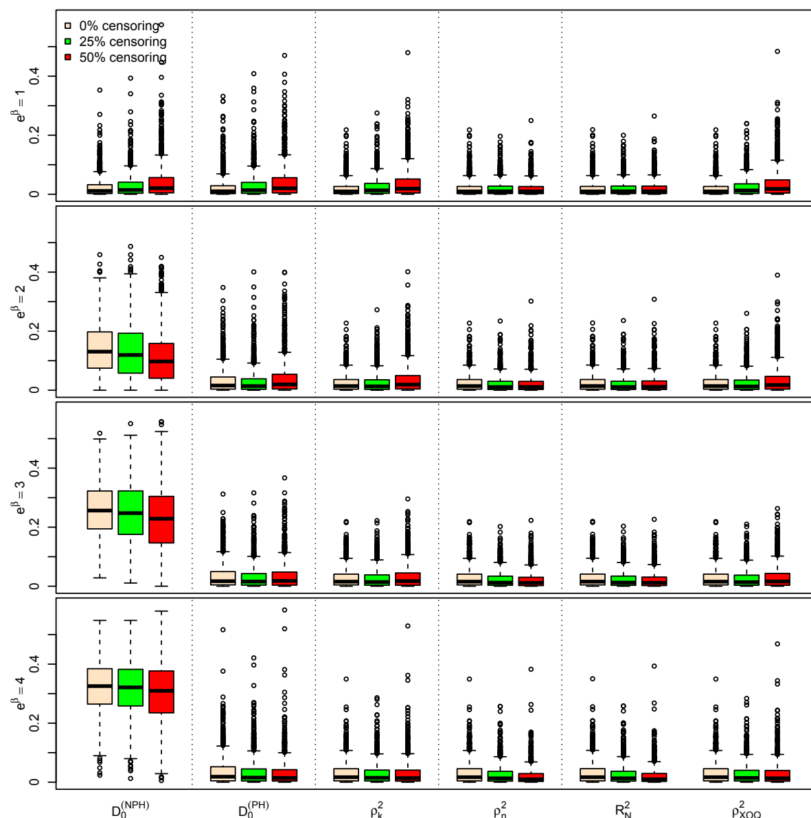
Figure 4 Simulations results for D_0^{(NPH)} , D_0^{(PH)} , \rho_k^2 , \rho_n^2 , R_N^2 and \rho_{XOQ}^2 , for n = 50 subjects, Z \sim B(1/2) , X \sim W(1, e^\beta Z) and a uniform censoring (1,000 repetitions). Boxplots of the different indices according to the values of e^\beta and p_c .
