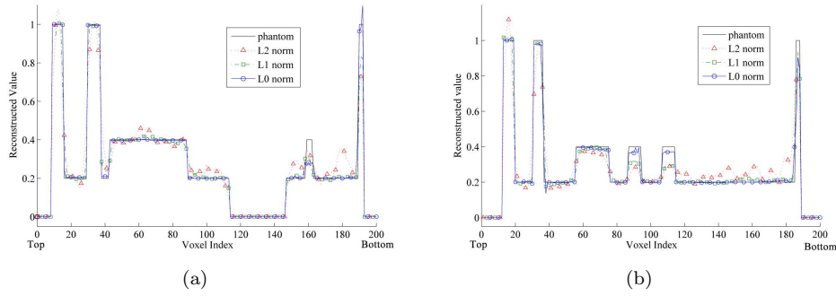
Figure 4. Intensity profile along the vertical lines placed in Fig 2.a (100th column, z = 0 mm) and 2.b ( 78th column, x = 0 mm). The black solid line corresponds to the ground truth, the dash lines with triangle, square and circle markers represent the L2 norm, L1 norm and L0 norm respectively.
