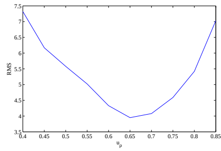
Figure 12. RMSE curve corresponding to different relaxation parameters.
