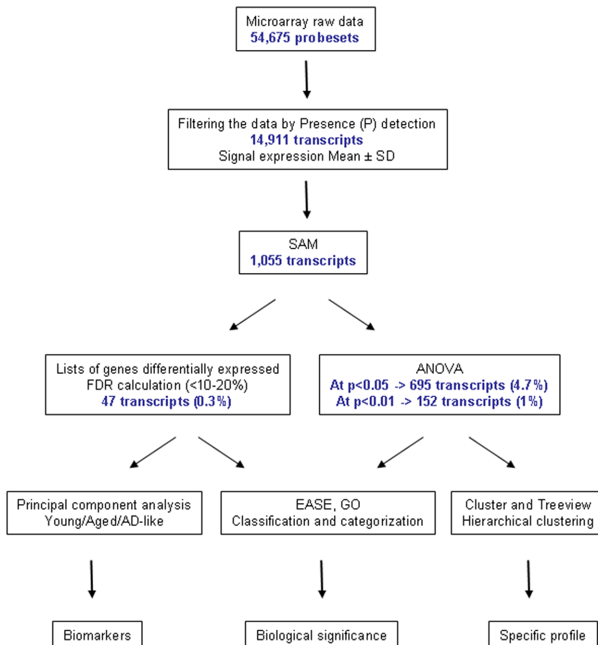
Figure 2. Schematic representation of the different analyses. Microarray data were filtered to detect the present transcripts (P). Then the filtered data were processed by SAM. ANOVA was performed with the (P) data and with the data sorted by SAM and the 47 P selected genes were analyzed by PCA. Finally, the 47 and the 695 genes were investigated by clustering and were classified by functional categories. doi:10.1371/journal.pone.0012770.g002
