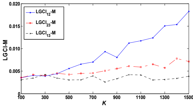
Fig. 3. LGCI-M with K varying from 100 to 1500.
