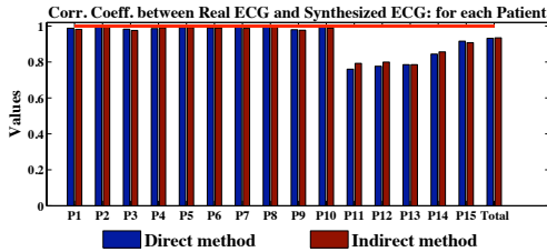
Figure 2. Correlation coefficient between real ECG and synthesized ECG, for each patient, using direct method and indirect method.
