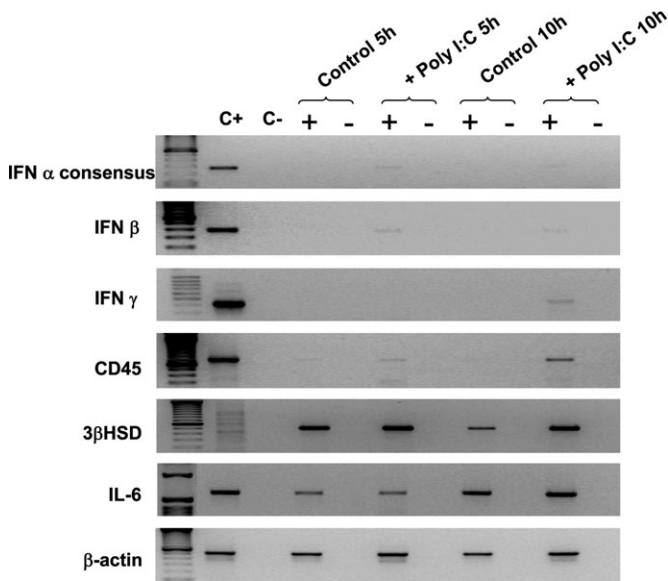
Figure 1: IFNs \alpha , \beta , \gamma and cell marker transcripts detection in Leydig cells. RT–PCR was performed to detect mRNAs encoding: a consensus region for the 12 human IFNs \alpha , IFN \beta , IFN \gamma , CD45 (haematopoietic cell marker), 3 \beta -HSD (Leydig cell marker), IL-6 (produced by Leydig cells) (all 35 cycles of PCR) and \beta -actin (30 cycles) in human Leydig cell cultures stimulated or not (control) for 5–10 h by poly I:C. For each mRNA sample, both a reverse transcriptase (RT) reaction (+) and a negative control reaction without RT (–) were performed (C+: positive control represented by PBMC stimulated 24 h by poly I:C; C–: negative control).
