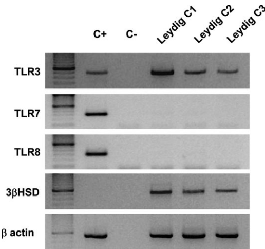
Figure 2: TLRs expression by human Leydig cells. RT–PCR was performed to detect mRNAs encoding TLR3, TLR7 and TLR8 in independent Leydig cell cultures from three donors (Leydig C1–3) (C+: positive control represented by PBMC stimulated for 24 h by poly I:C; C–: negative control).
