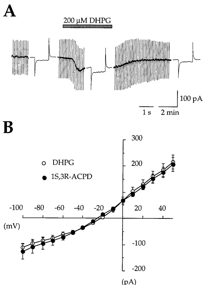
Figure 5. The group I mGluRs selective agonist DHPG (200 \mu M) evoked a CAN current identical to that evoked by 1S,3R-ACPD. A , Membrane current and conductance changes evoked by DHPG (200 \mu M, 2 min, V_H = -60 mV). B , Mean I/V relations of DHPG-induced ( \circ ) and 1S,3R-ACPD-induced ( \bullet ) currents ( n = 5 ; paired data). Note that I/V relations are very similar (reversal potential, slope conductance; but see also Table 1).
