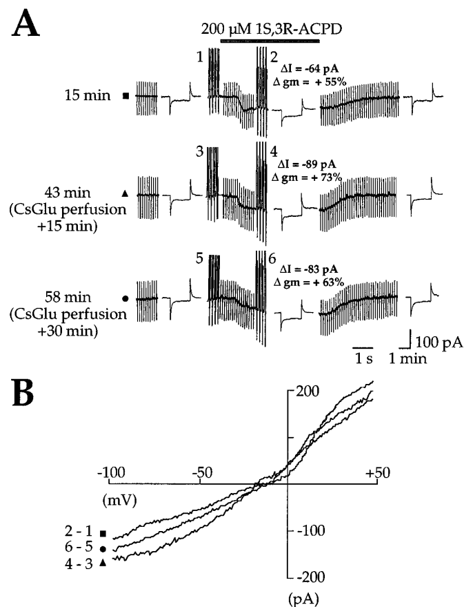
Figure 3. Intracellular perfusion with control CsGlu pipette solution does not modify I_{\text{CAN}} . A , Membrane currents ( \Delta I ) and conductance changes ( \Delta gm ) evoked in the same cell by three successive applications of 1S,3R-ACPD (200 μM, 2 min, V_H = -60 mV) in control (■), after 15 min of cell dialysis with the control CsGlu pipette solution (▲), and after 30 min of cell dialysis with the control CsGlu pipette solution (●). Note that the successive applications of 1S,3R-ACPD induced three similar I_{\text{CAN}} . B , I/V relations of the CAN currents induced, in the same cell, by three successive 1S,3R-ACPD applications and performed, respectively, before (■), 15 (▲), and 30 min (●) after pipette-whole-cell perfusion with control CsGlu pipette solution. These I/V relations have been obtained by subtracting the current traces at the time indicated by the numbers in A .
