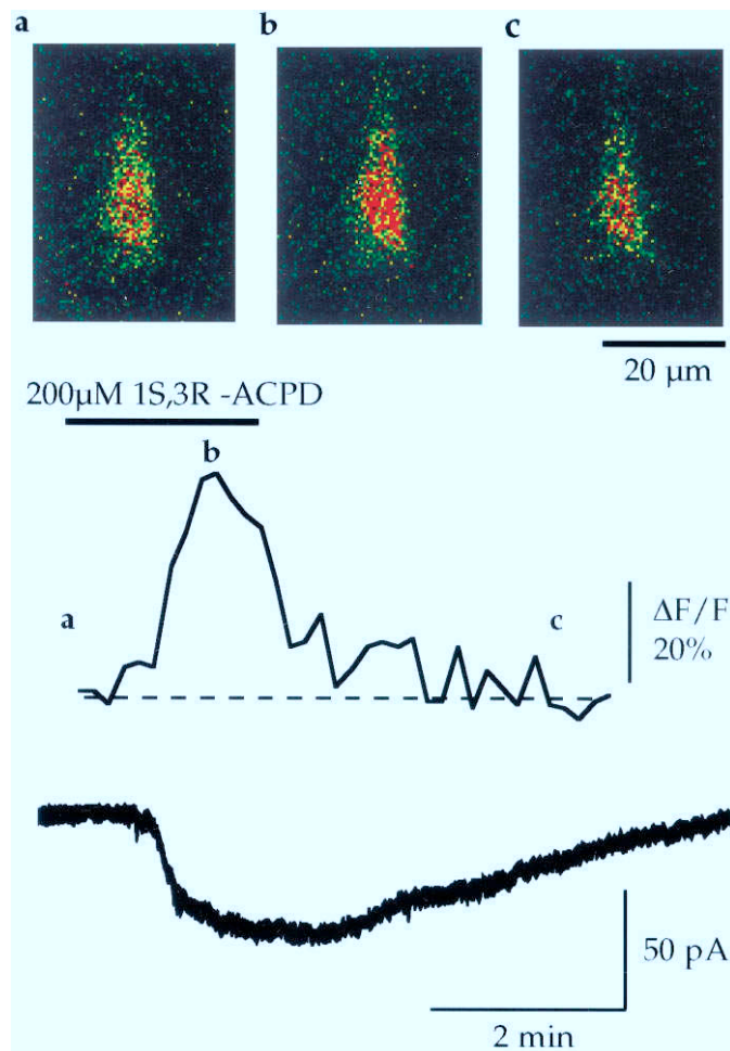
Figure 2. I_{\text{ACPD}} is associated with an increase in intracellular [\text{Ca}^{2+}] . Changes in intracellular [\text{Ca}^{2+}] induced by application of 1S,3R-ACPD were recorded from the soma of CA1 pyramidal neurons loaded in whole-cell configuration with the \text{Ca}^{2+} -sensitive dye Fluo-3 (0.01 mM diluted in the CsGlu pipette solution). Fluorescence images were acquired every 10 sec; [\text{Ca}^{2+}]_i was quantified and correlated to the simultaneously recorded CAN current. Top panels , Successive pseudocolored photomicrographs of the fluorescence collected before ( a ), during ( b ), and after ( c ) application of 1S,3R-ACPD (200 μM, 2 min, V_H = -60 mV). Middle trace , Mean changes of the \text{Ca}^{2+} -dependent fluorescence, observed in four CA1 pyramidal neurons, during the corresponding electrophysiologically recorded I_{\text{CAN}} ( bottom trace ). Note that the rise in [\text{Ca}^{2+}]_i is strictly correlated to the rise phase of I_{\text{CAN}} .
