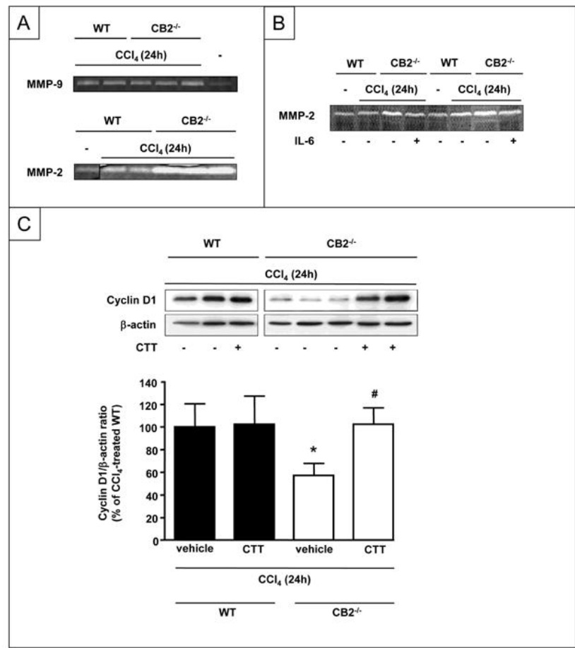
Figure 7 CB2 receptor inactivation delays liver regeneration by a mechanism involving enhanced MMP-2 activity Gelatin zymography showing (A) MMP-9 and MMP-2 activities and (B) MMP-2 activities of liver homogenates from WT and CB2 -/- mice injected with IL-6 or vehicle and sacrificed 24 h after CCl 4 administration. (C) Representative western blot of hepatic cyclin D1 expression 24 h after CCl 4 injection, following CTT or vehicle treatment. *P <0.05 for CTT vs vehicle.
