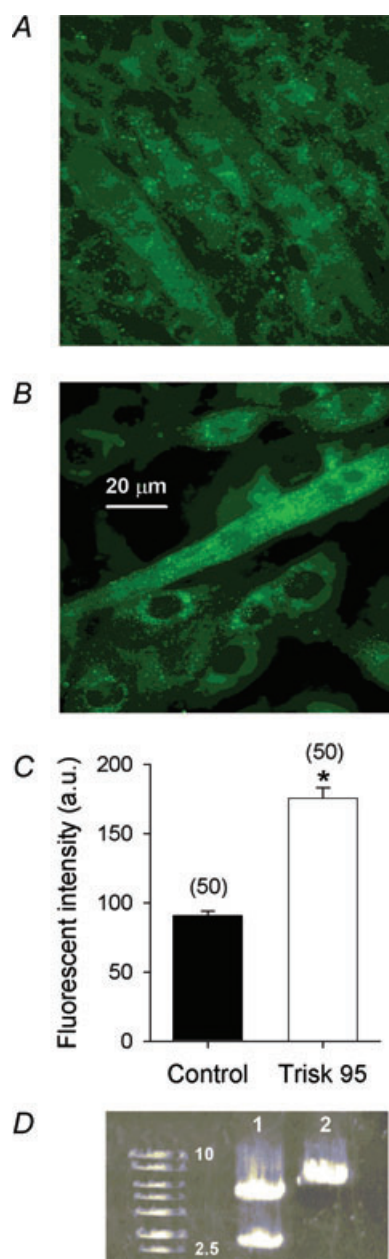
Figure 1. Overexpression of Trisk 95 in C2C12 cells
