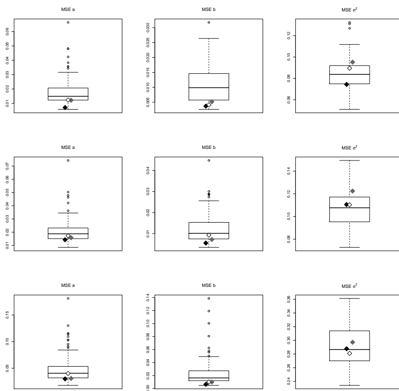
FIG 3. Box-plot of the MSE_{f_s} of all possible fixed choices together with the MSE_{m_s} of both criteria in Model 3 with a = 0 , b = 0.5 and \sigma^2 = 1/8 (1 st line), \sigma^2 = 1/4 (2 nd line) or \sigma^2 = 1/2 (3 rd line), for g(\theta) = a (left) and g(\theta) = b (middle), g(\theta) = \sigma^2 (right); black diamond for the first criterion, white diamond for the second criterion and grey diamond for the third criterion in modulated strategy.
