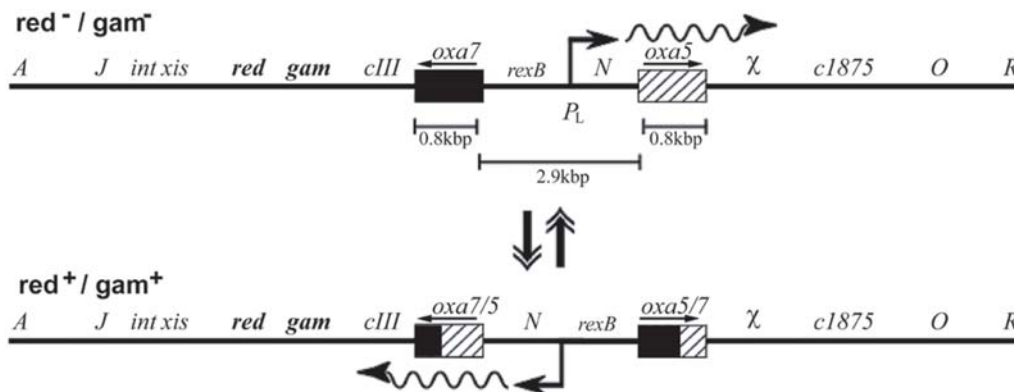
Figure 1. Recombination between the two homeologous oxa sequences flanking the \lambda pL promoter leads to a phenotypic switch. In \lambda red- gam- , transcription from the pL promoter proceeds rightward and the red and gam genes are not transcribed. Recombination between the two homeologous sequences leads to inversion of the pL-N segment causing a selectable phenotype (see Text for details). Not drawn to scale. doi:10.1371/journal.pgen.1000065.g001
