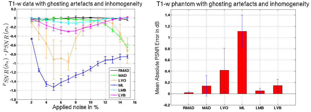
Fig. 10. Result of the denoising experiment. Left: difference in dB between the PSNR obtained with the estimation provided by automatic methods \hat{\sigma}_n and the PSNR obtain with the truth \sigma_n . Right: mean absolute difference in dB between \text{PSNR}(\sigma_n) and \text{PSNR}(\hat{\sigma}_n) .
